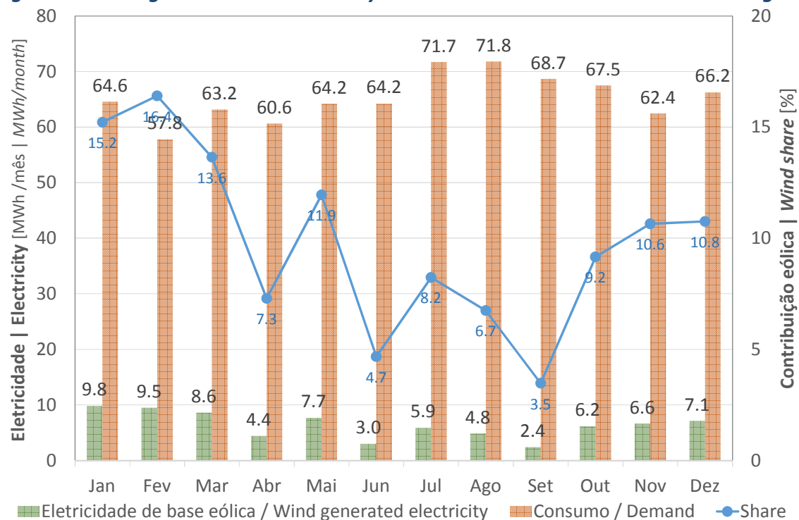
Figure 10: Wind generation vs. Electricity demand 2015 - Madeira Autonomous Region
