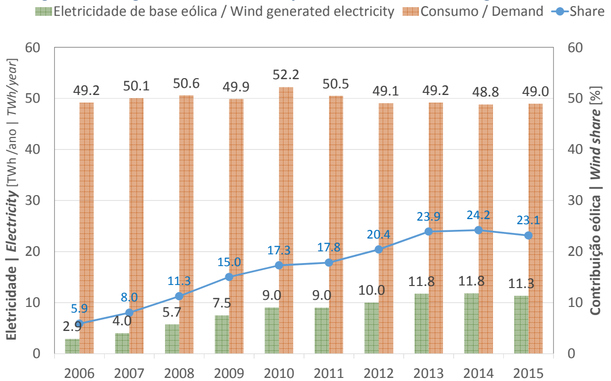
Figure 7: Wind generation vs. Electricity demand 2006-2015 - Portugal Mainland
