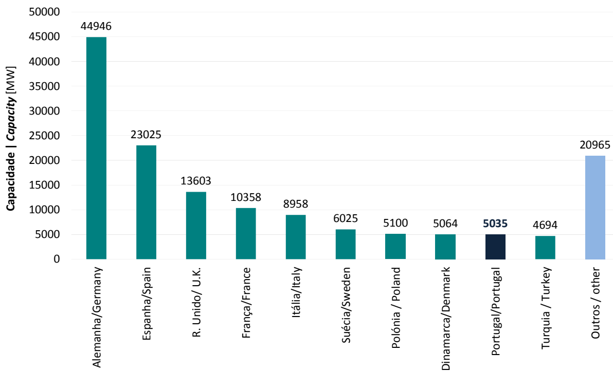
Figure 2: Installed capacity 2015 - Europe
