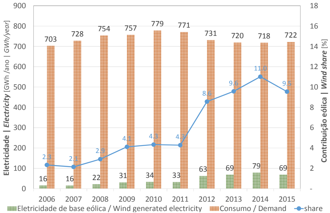
Figure 11: Wind generation vs. Electricity demand 2006-2014 - Azores Autonomous Region
