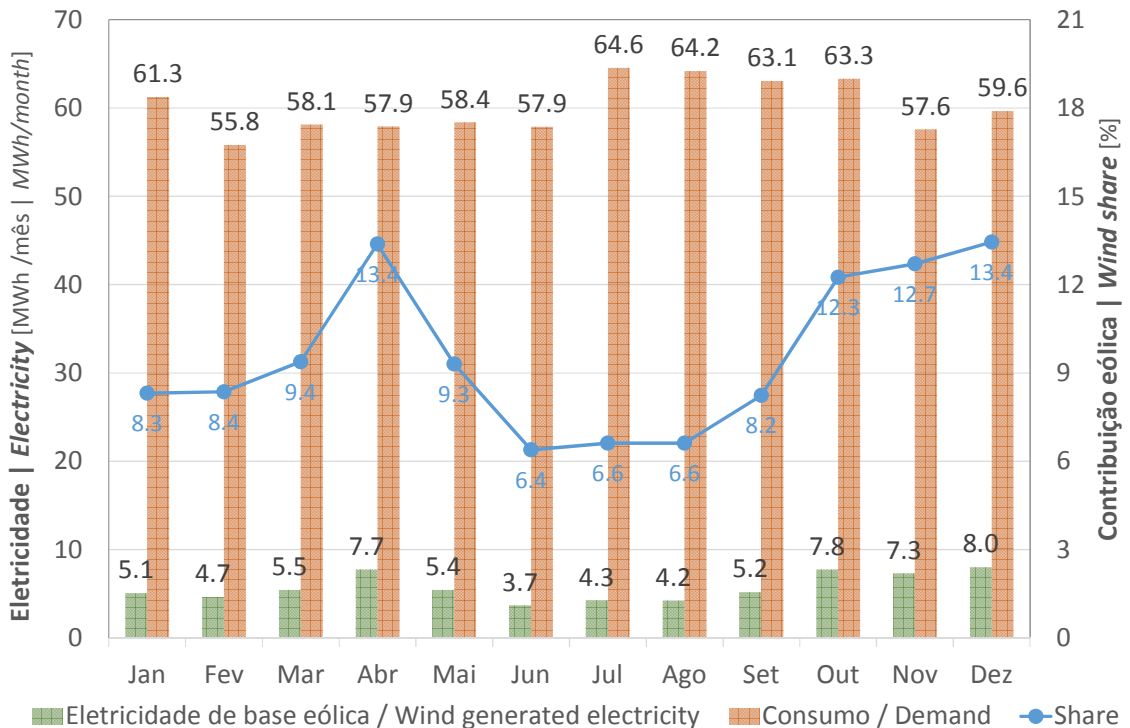
Figure 12: Wind generation vs. Electricity demand 2015 - Azores Autonomous Region
