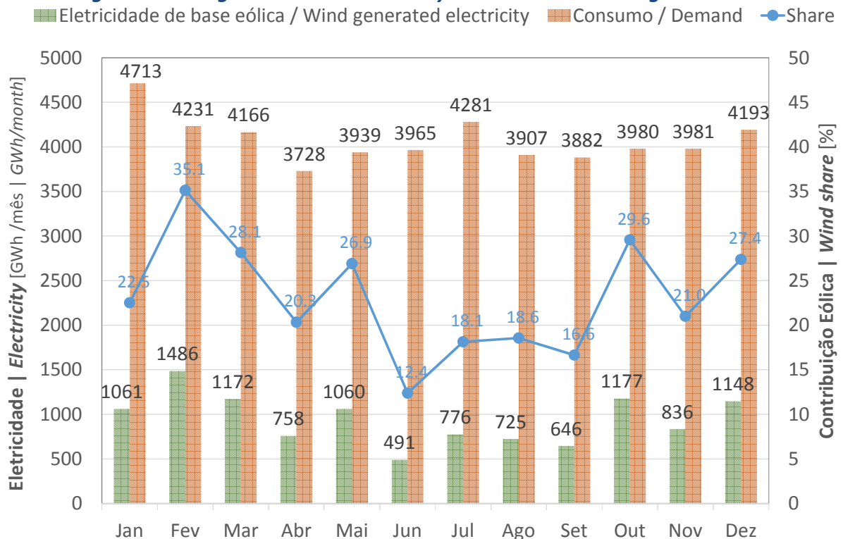
Figure 8: Wind generation vs. Electricity demand 2015 - Portugal Mainland
