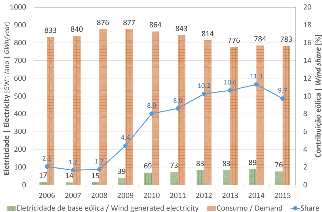
Figure 9: Wind generation vs. Electricity demand 2006-2015 - Madeira Autonomous Region
