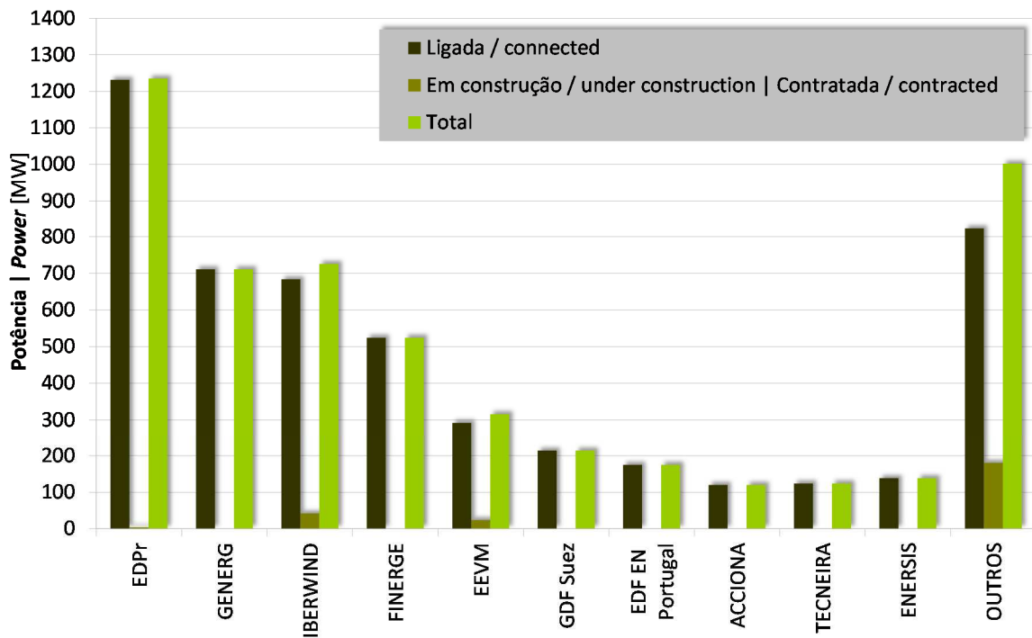
Figura 20: Promotores 2015 Figure 20: Developers 2015
