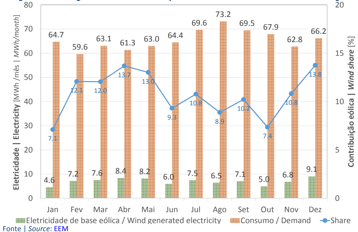
Figure 10: Wind generation vs. Electricity demand 2016 - Madeira Autonomous Region
