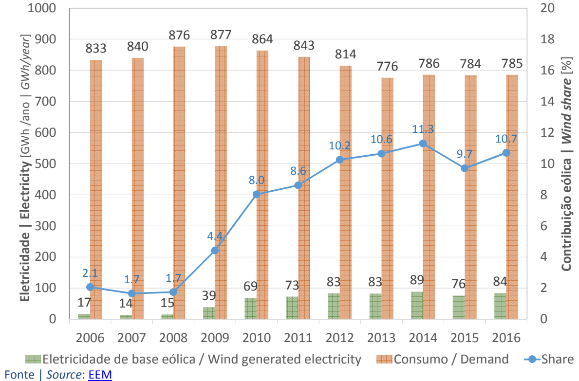
Figure 9: Wind generation vs. Electricity demand 2006-2016 - Madeira Autonomous Region
