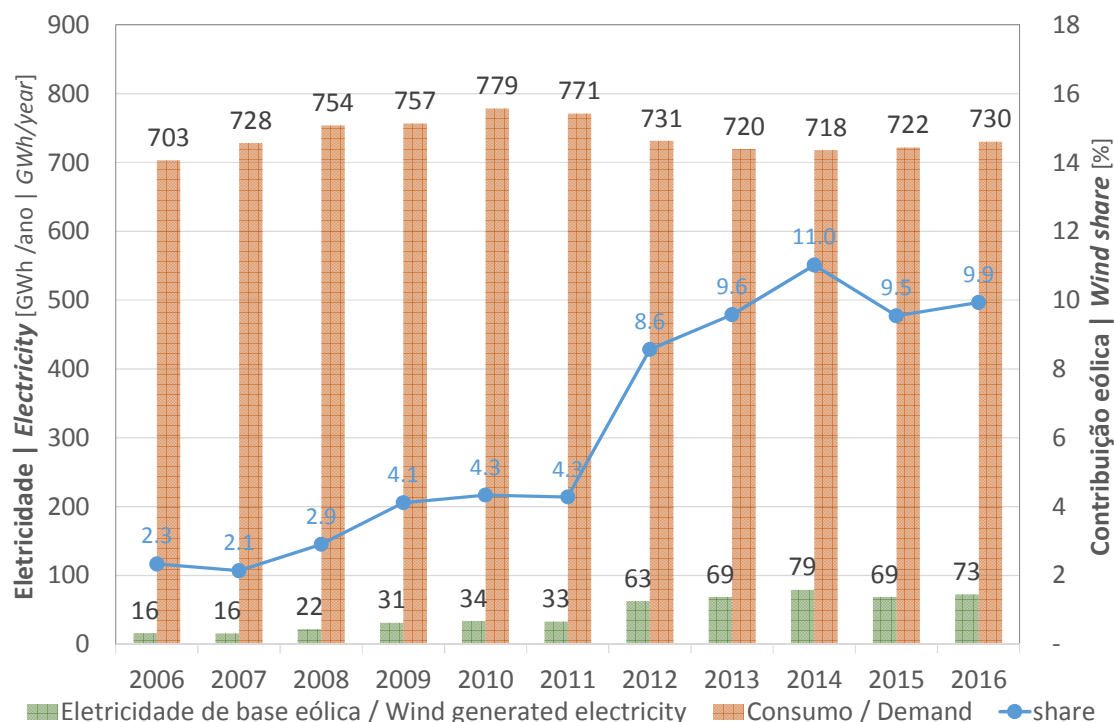
Figure 11: Wind generation vs. Electricity demand 2006-2016 - Azores Autonomous Region
