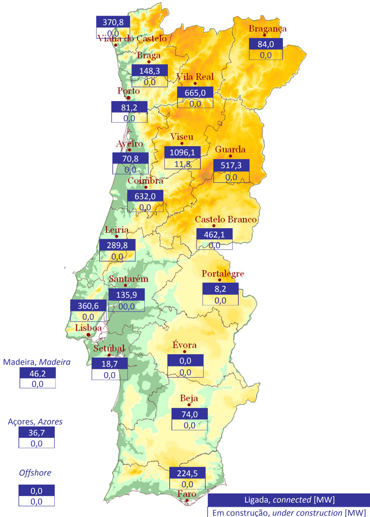
Figure 14: Installed capacity per district and autonomous region 2016 – Portugal Mainland
