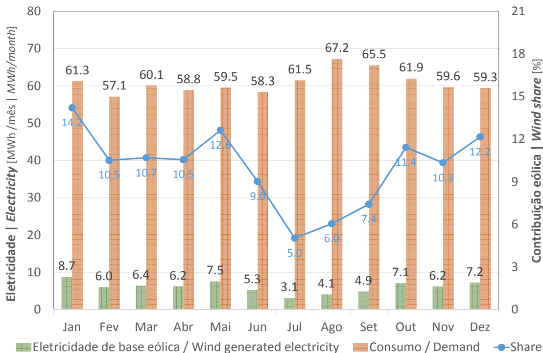
Figure 12: Wind generation vs. Electricity demand 2016 - Azores Autonomous Region
