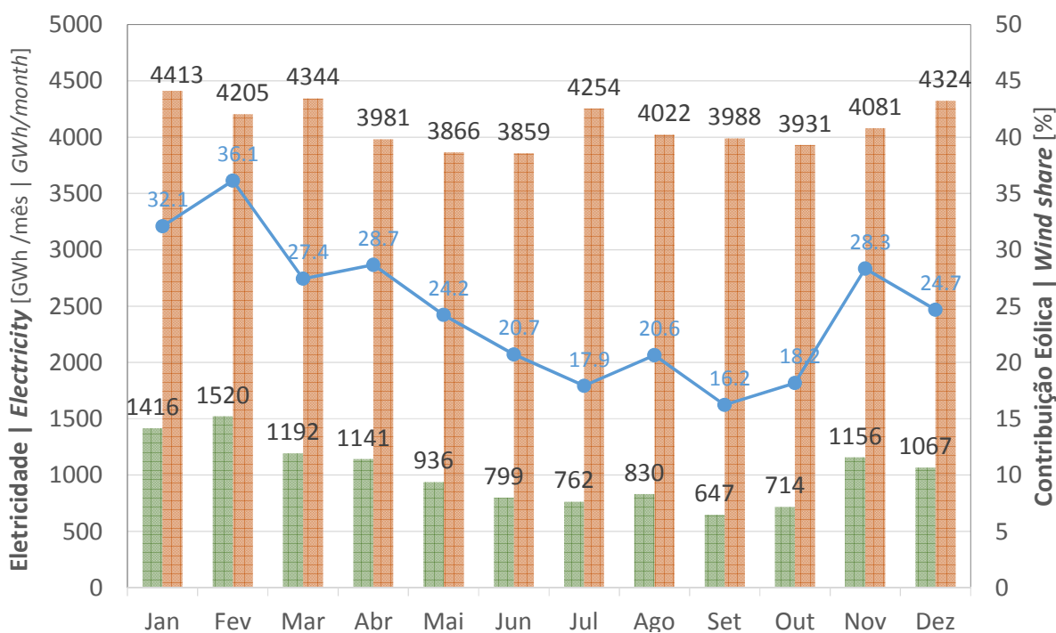
Figure 8: Wind generation vs. Electricity demand 2016 - Portugal Mainland
