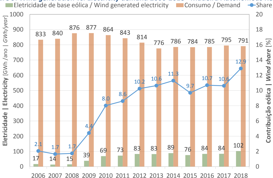
Figure 9: Wind generation vs. Electricity demand 2006-2018 - Madeira Autonomous Region
