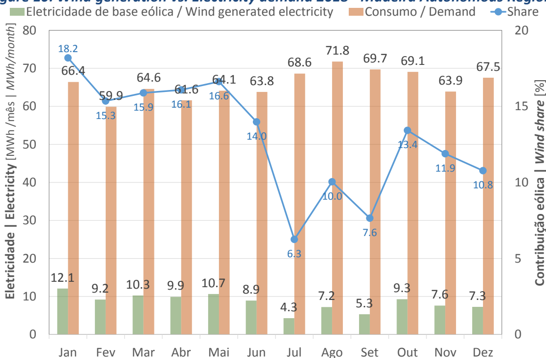
Figure 10: Wind generation vs. Electricity demand 2018 - Madeira Autonomous Region
