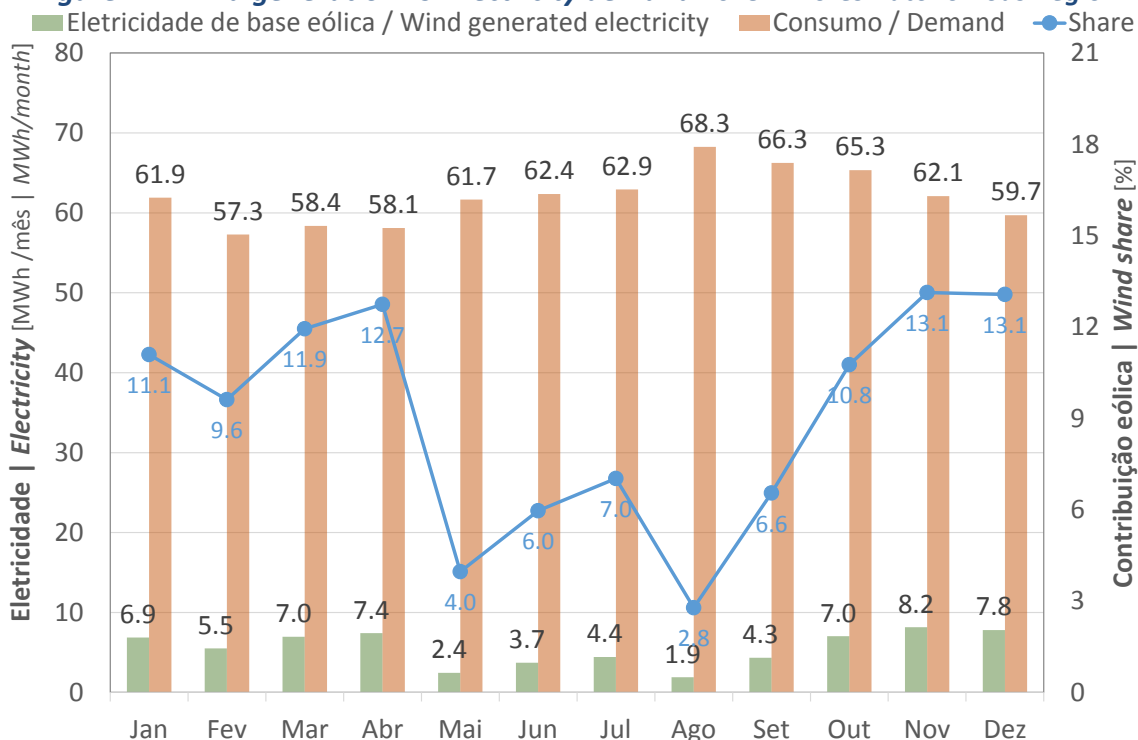
Figure 12: Wind generation vs. Electricity demand 2018 - Azores Autonomous Region
