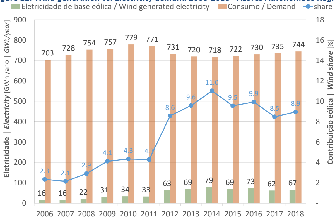
Figure 11: Wind generation vs. Electricity demand 2006-2018 - Azores Autonomous Region
