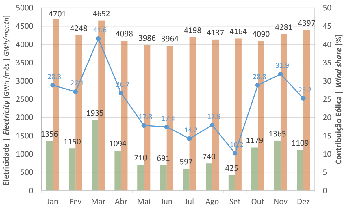
Figure 8: Wind generation vs. Electricity demand 2018 - Mainland Portugal
