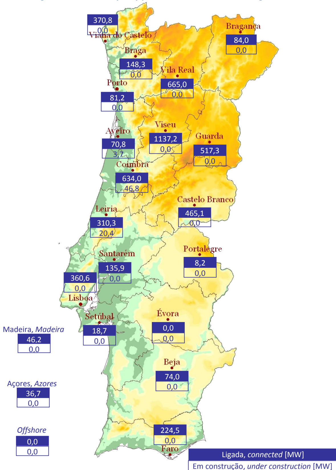
Figure 14: Installed capacity per district and autonomous region 2018
