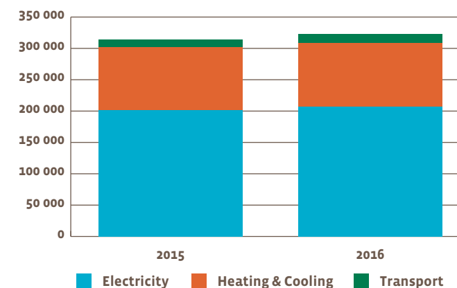
Avoided fossil fuels per sector (ktoe)
