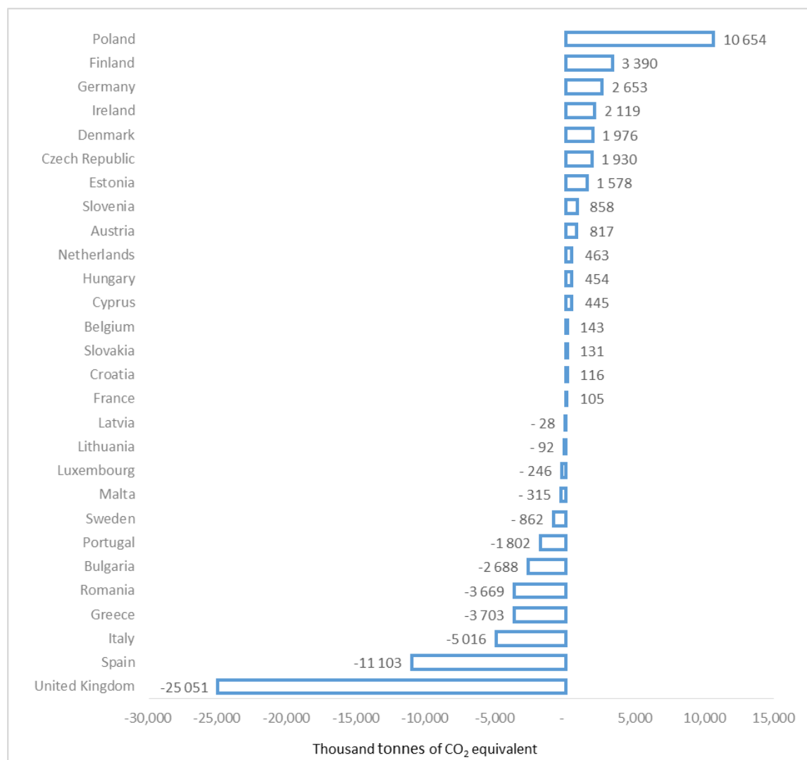
Figure 2: Change in total GHG emissions by EU Member State, 2015-2016
