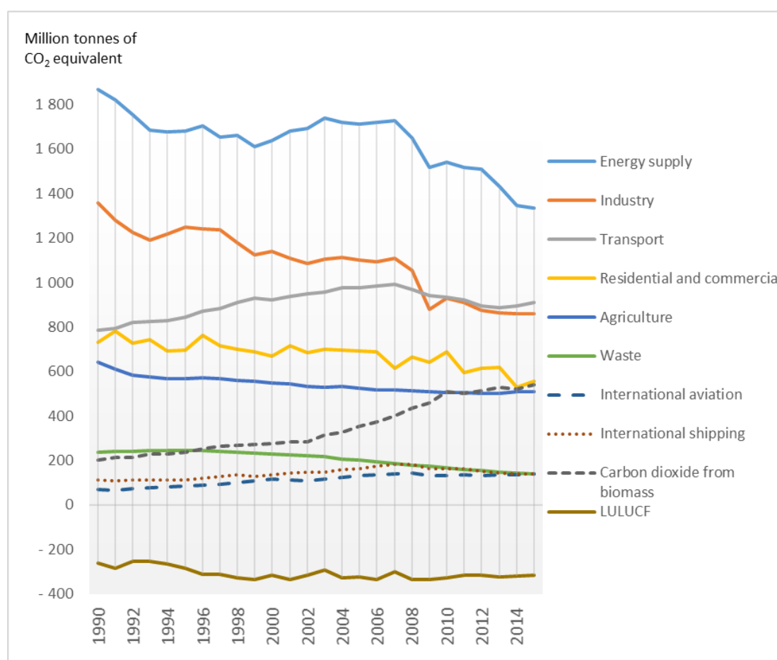
Figure 3: GHG emissions by sector in the EU-28
