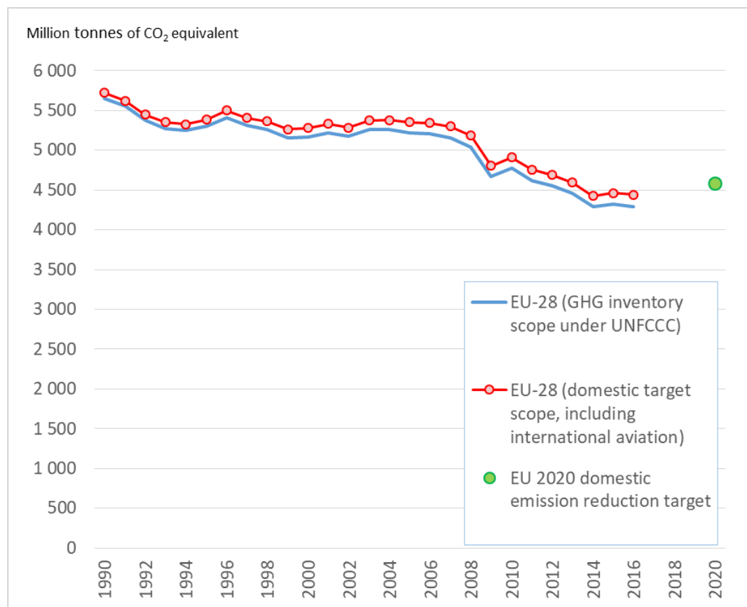
Figure 1: Total GHG emissions, 1990-2016
