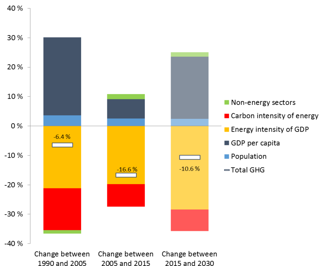
Figure 4: Decomposition analysis of key historic and projected emission drivers in the EU, 1990-2030
