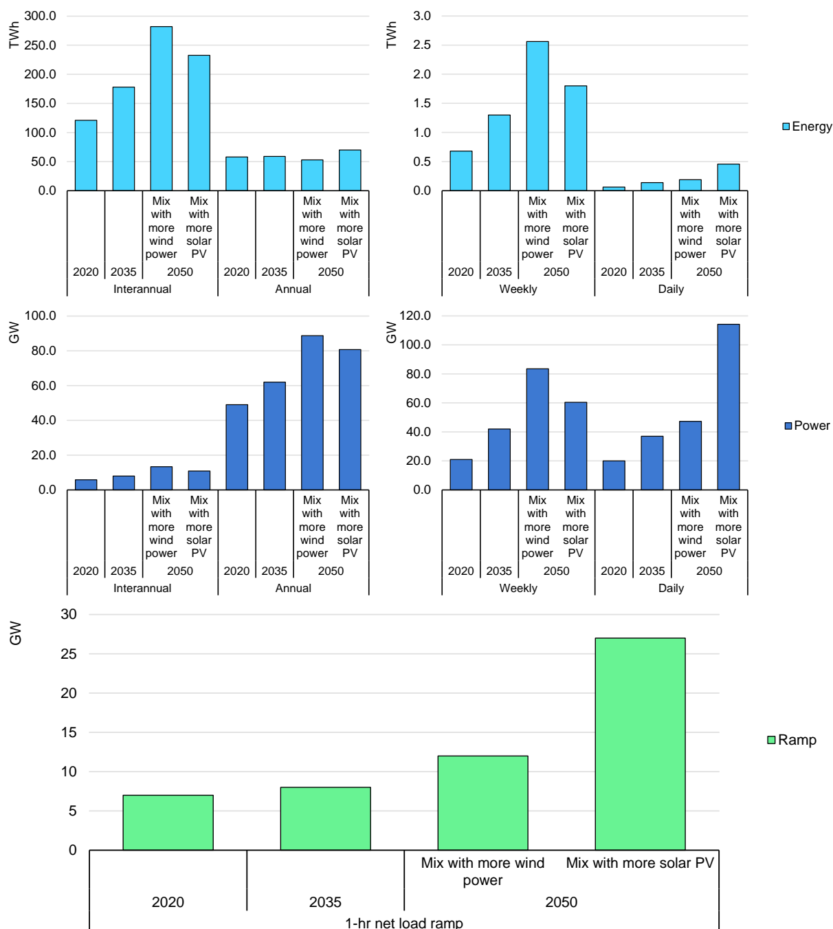
Figure 5.2 Flexibility needs in energy and power of the French Multi-Ancual Energy Plan to 2035 and National Low-Carbon Strategy to 2050 with different renewable mixes, compared with today's values over 200 meteorological conditions
