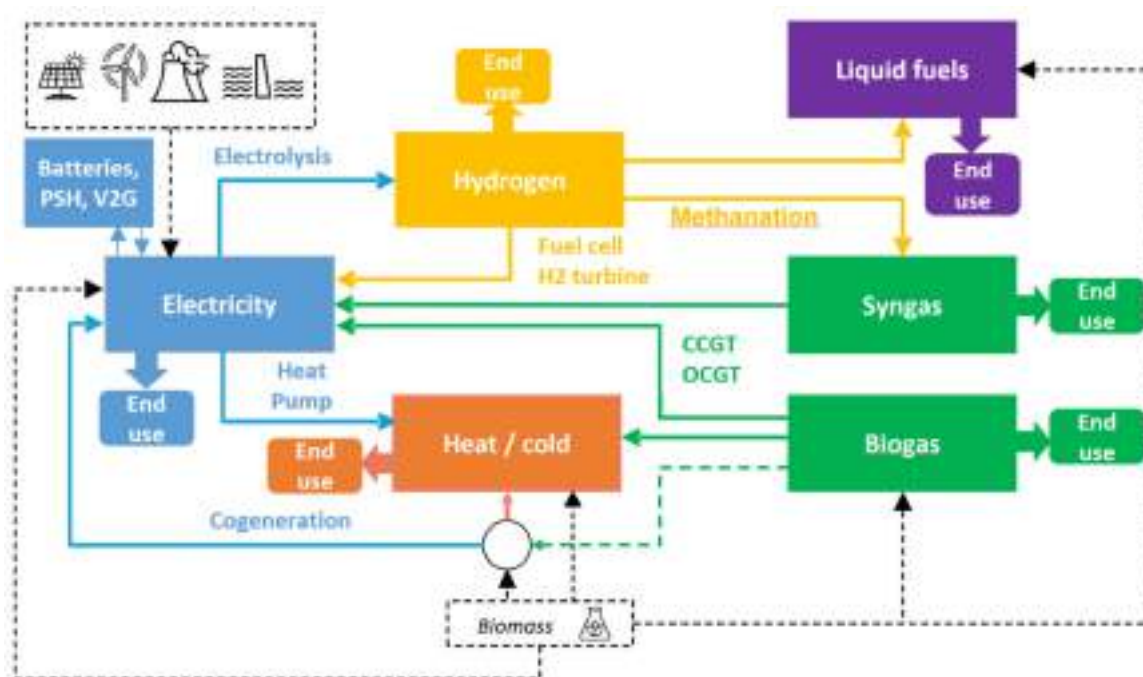
Figure 5.7 Couplings of the power system with other energy carriers
