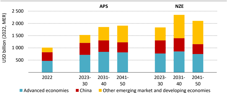
Figure 3.1 ▶ Average annual investment in clean power sector technologies by region and scenario
