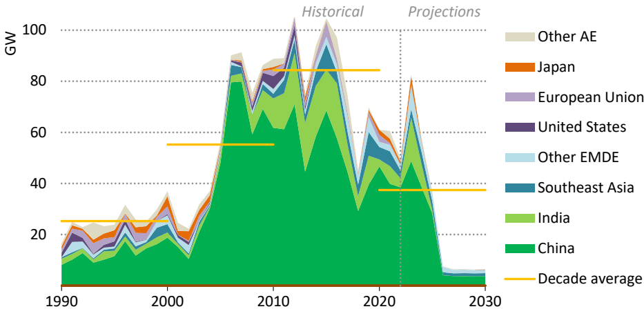
Figure 2.1 ▶ Global coal-fired capacity additions in the APS
