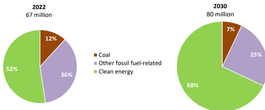
Figure 4.3 ▶ Global energy sector employment by fuel in the APS
