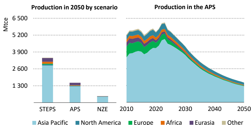
Figure 1.5 ▶ Coal production by country/region and scenario
