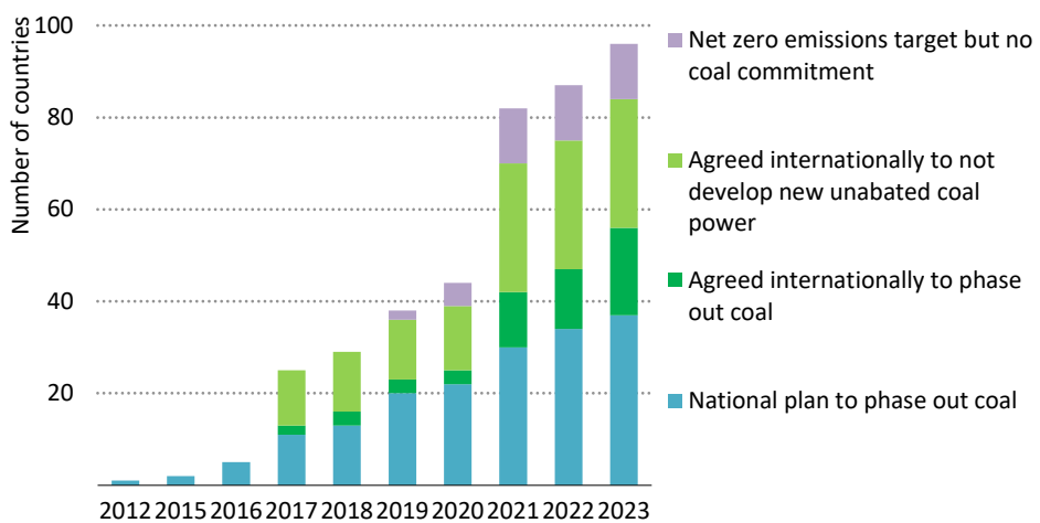
Figure 1.8 ▶ Number of countries with plans to phase down coal use and net zero emissions pledges
