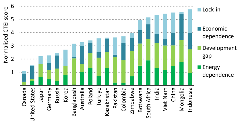
Figure 1.10 ▸ Coal Transitions Exposure scores, 2022
