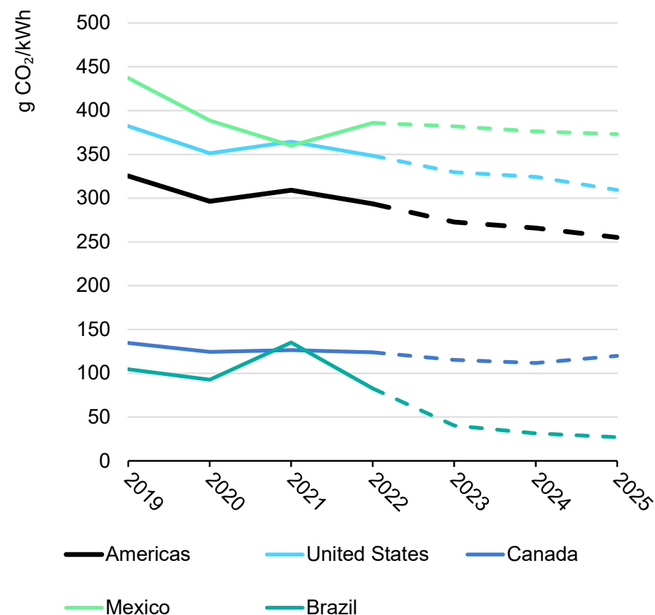
Development of average CO 2 intensity, Americas, 2019-2025
