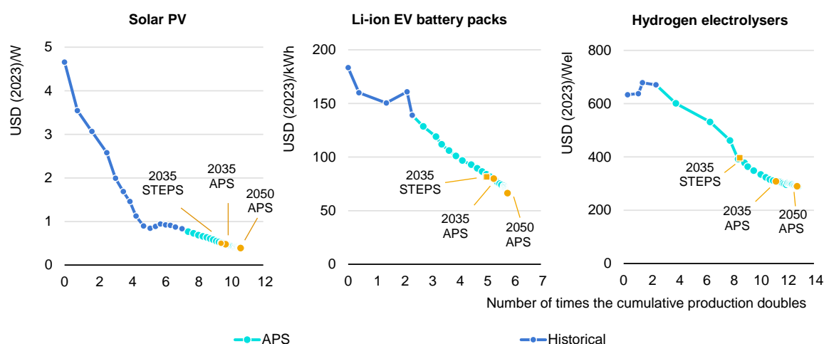
Figure 6.9 Global average production cost by number of doublings of cumulative deployment of selected technologies by scenario
