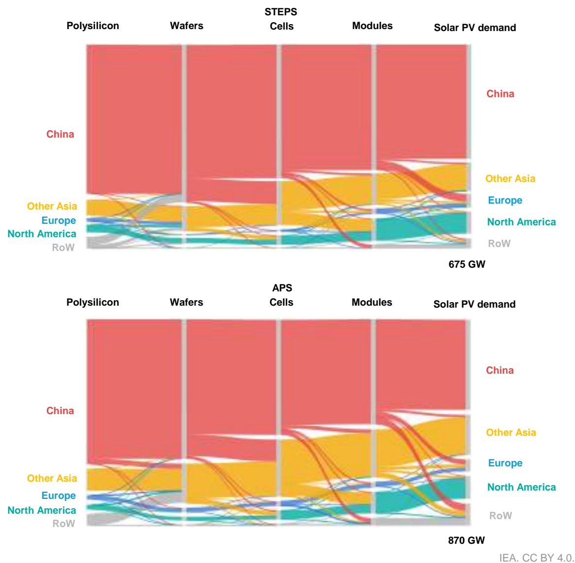
Figure A.8 Global manufacturing and trade flows of solar PV modules and components, Stated Policies Scenario and Announced Pledges Scenario, 2035
