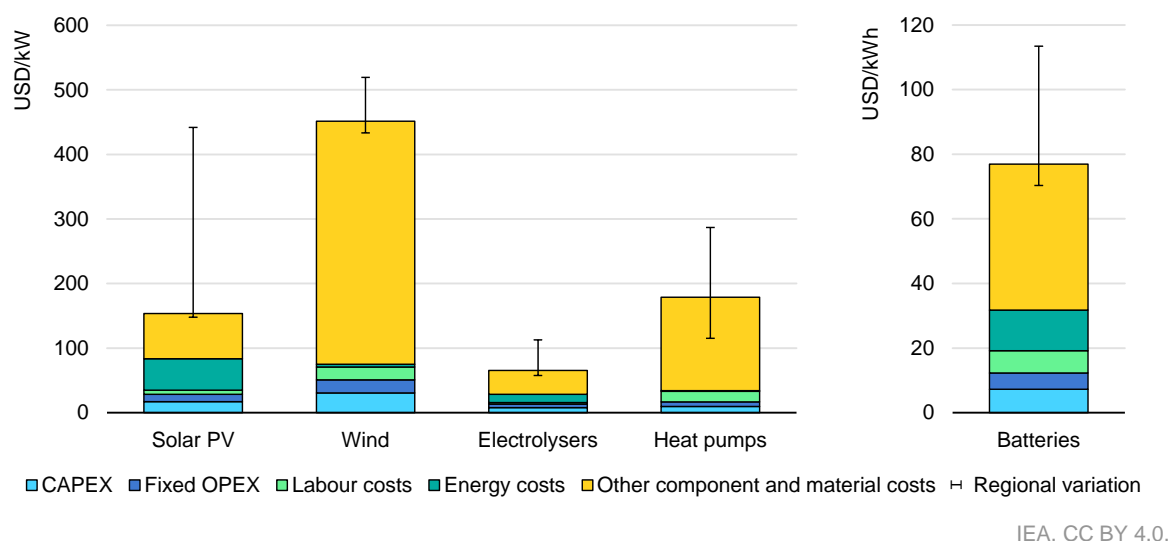
Figure 1.24 Global average levelised cost of production by cost factor for selected clean energy technologies and regional variation, 2023
