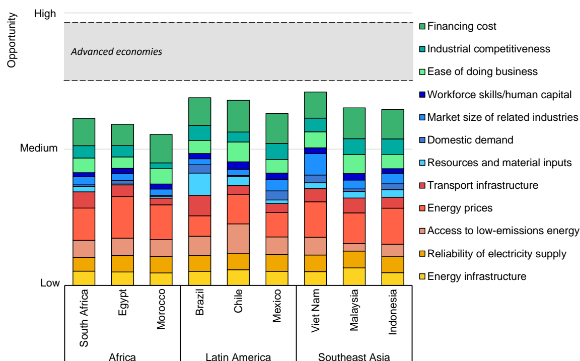
Figure 4.27 Top three scoring countries for enabling factors for iron and steel production in Africa, Latin America and Southeast Asia
