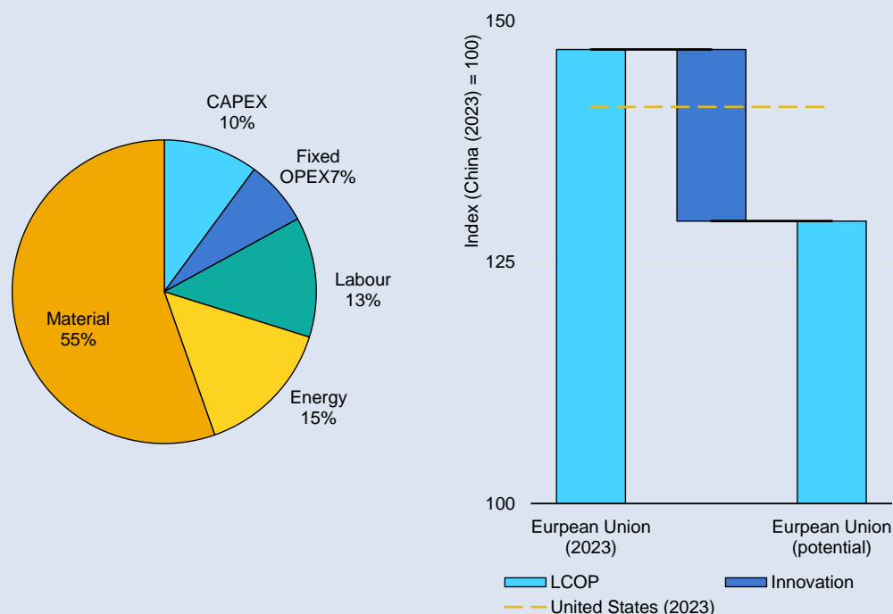
Figure 3.22 Global average battery levelised cost of production per cost factor and potential impact of innovation on battery costs in the European Union, 2023
