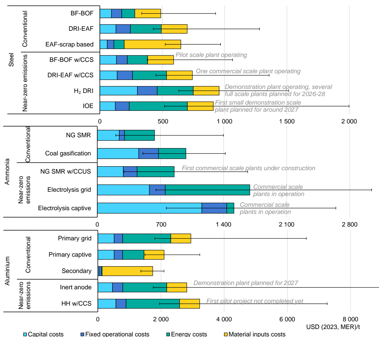
Figure 1.27 Levelised cost of production for selected materials by technology
