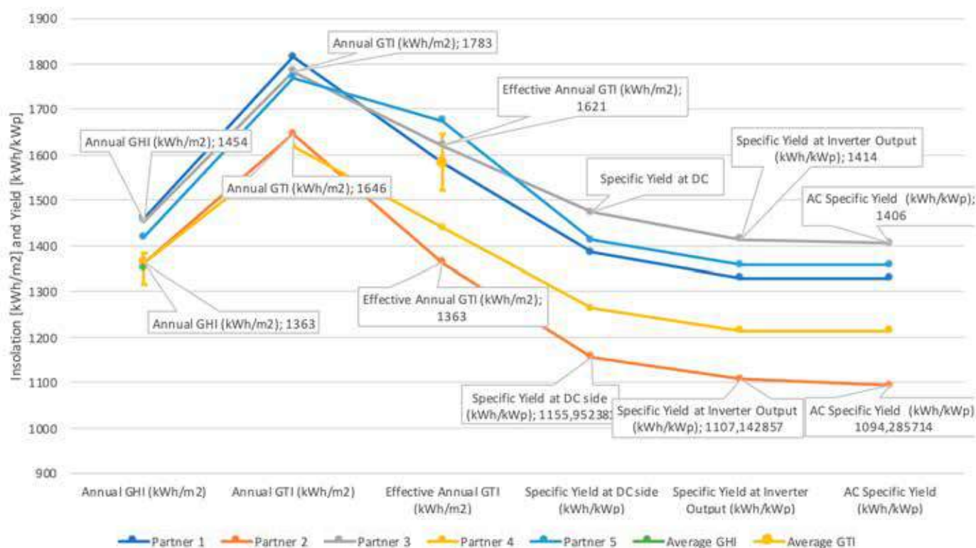
Fig. 3 - Detailed analysis of the contribution of each yield assessment modelling step from GHI to Alternating Current (AC) specific yield for the Bolzano site. The orange dots represent measured values over 2011-2019 with \sigma .
