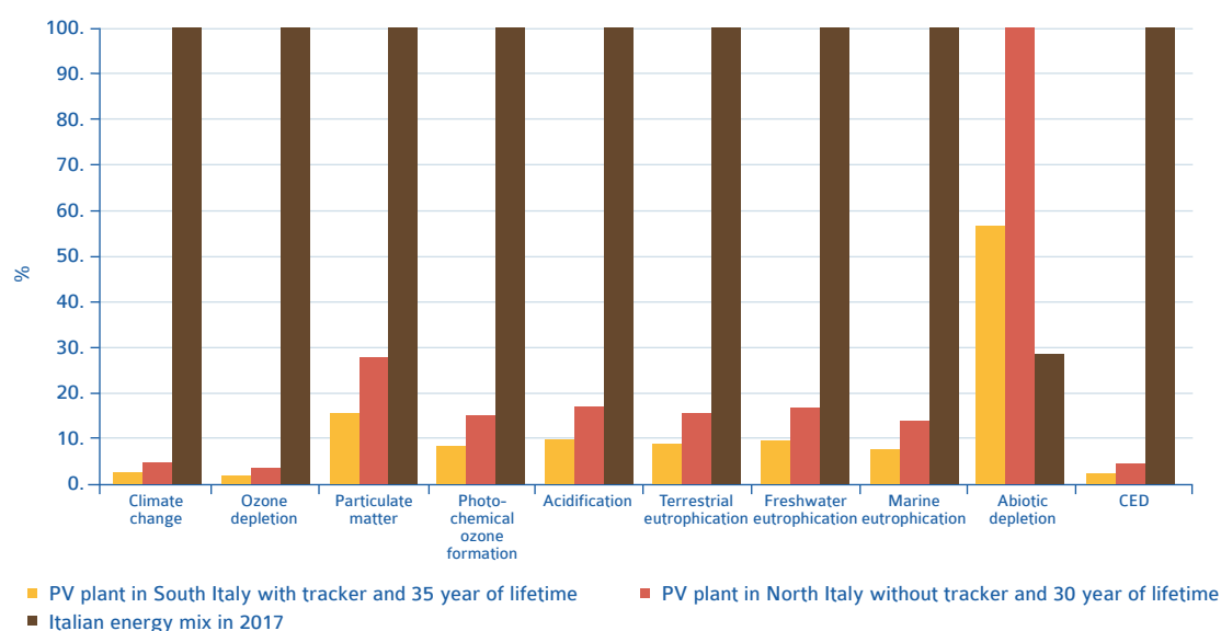
Fig. 5 - Comparison among the environmental impacts calculated by LCA for Italian energy mix and for two PV plants using HJT cell technology, in their best case (installation with tracker in southern Italy and with a useful life of 35 years) and in their worst case (installation on fixed plane in northern Italy and with a useful life of 30 years).
