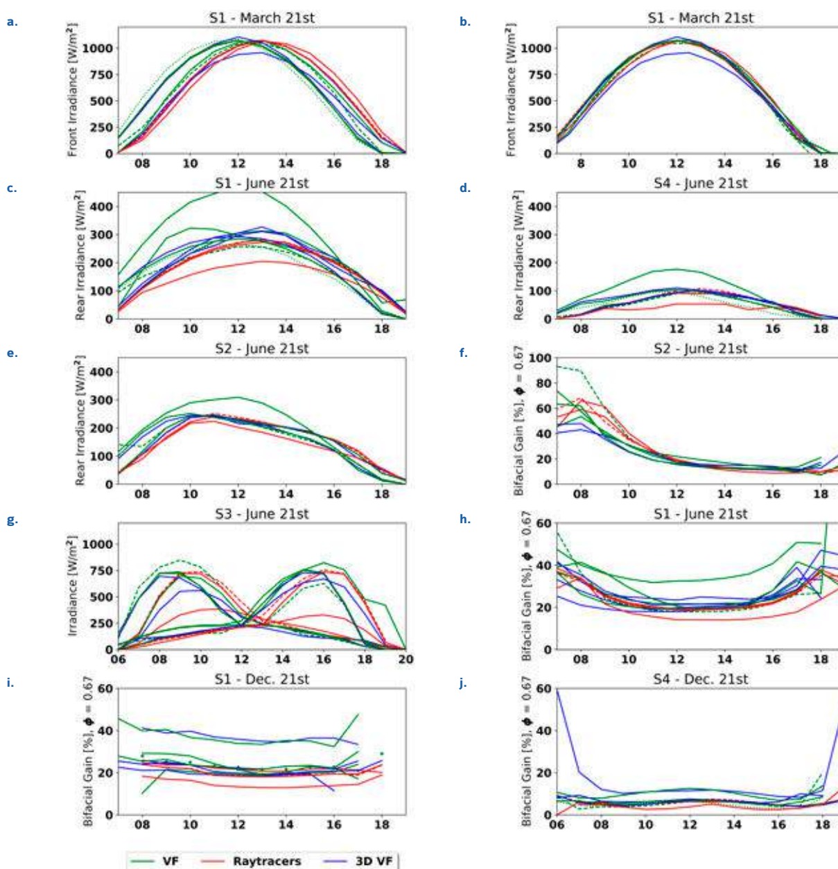
Fig. 2 - Example of modelling results run by ST1.2 experts for scenarios (S1-S4). The three model classes are denoted by colour: view factor models (green), raytracing models (red) and 3D VF and others (blue).
