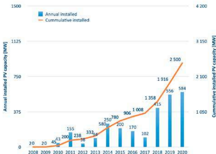
Fig. 1 - Development of grid-connected PV capacity in Israel through 2020.
