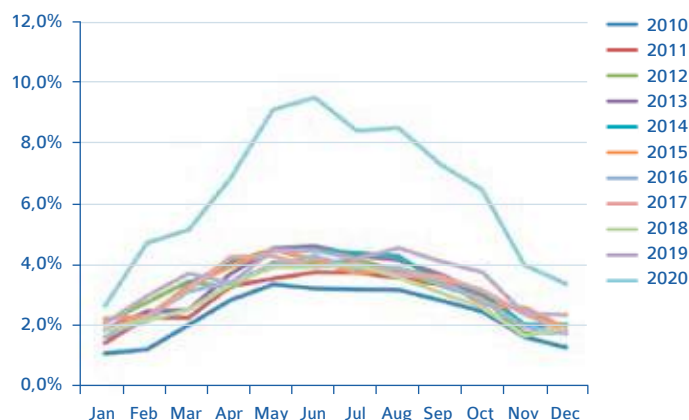
Fig. 3 - Monthly demand coverage by PV (last 11 years).
