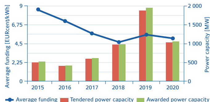
Fig. 1 – Average funding awarded in the auctions for ground-mounted PV installations.
