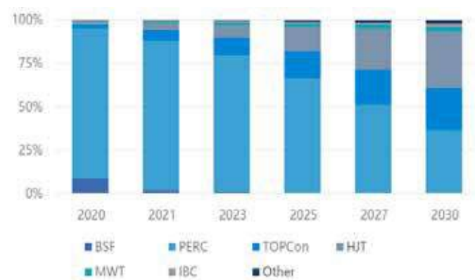
Fig. 5 - Forecast of China technological evolution (Source: CPIA).
