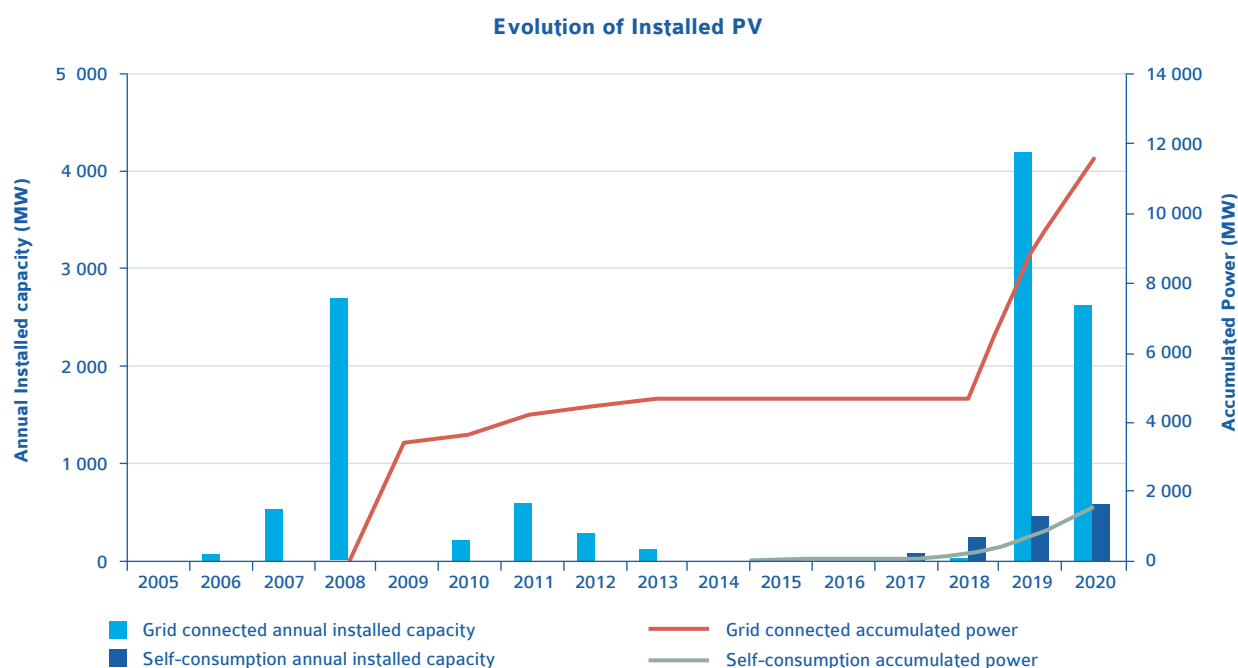
Fig. 5 - Evolution of installed PV 2005 – 2020, including grid-connected and self-consumption.
