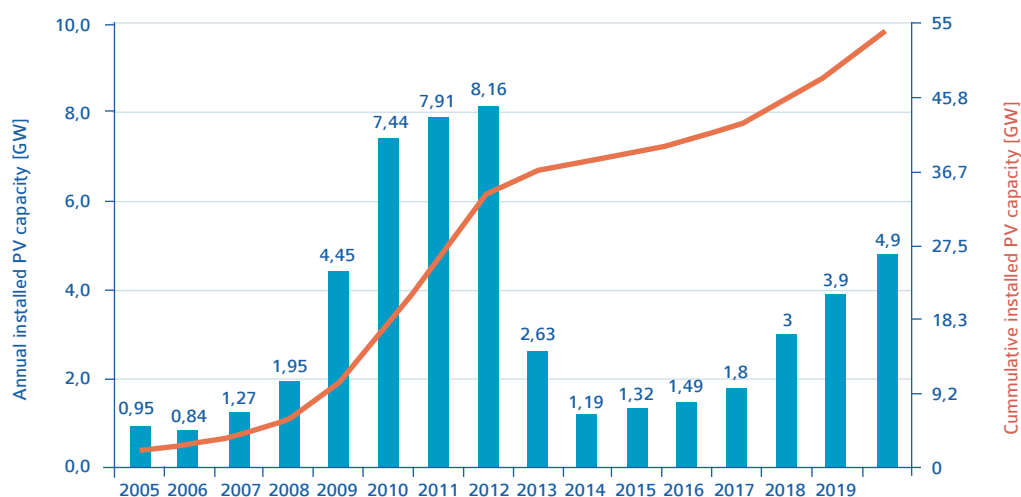
Fig. 5 - Development of grid connected PV capacity in Germany, *first estimate as of January 2021.
