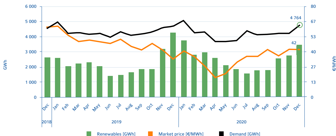
Fig. 3 - Renewable Electricity Production and Iberian Wholesale Electricity Market Price (December 2018 to December 2019) (Source: OMIE, REN; APREN's analysis).
