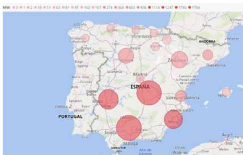
Fig. 6 - Geographical distribution of PV capacity installed in Spain.
