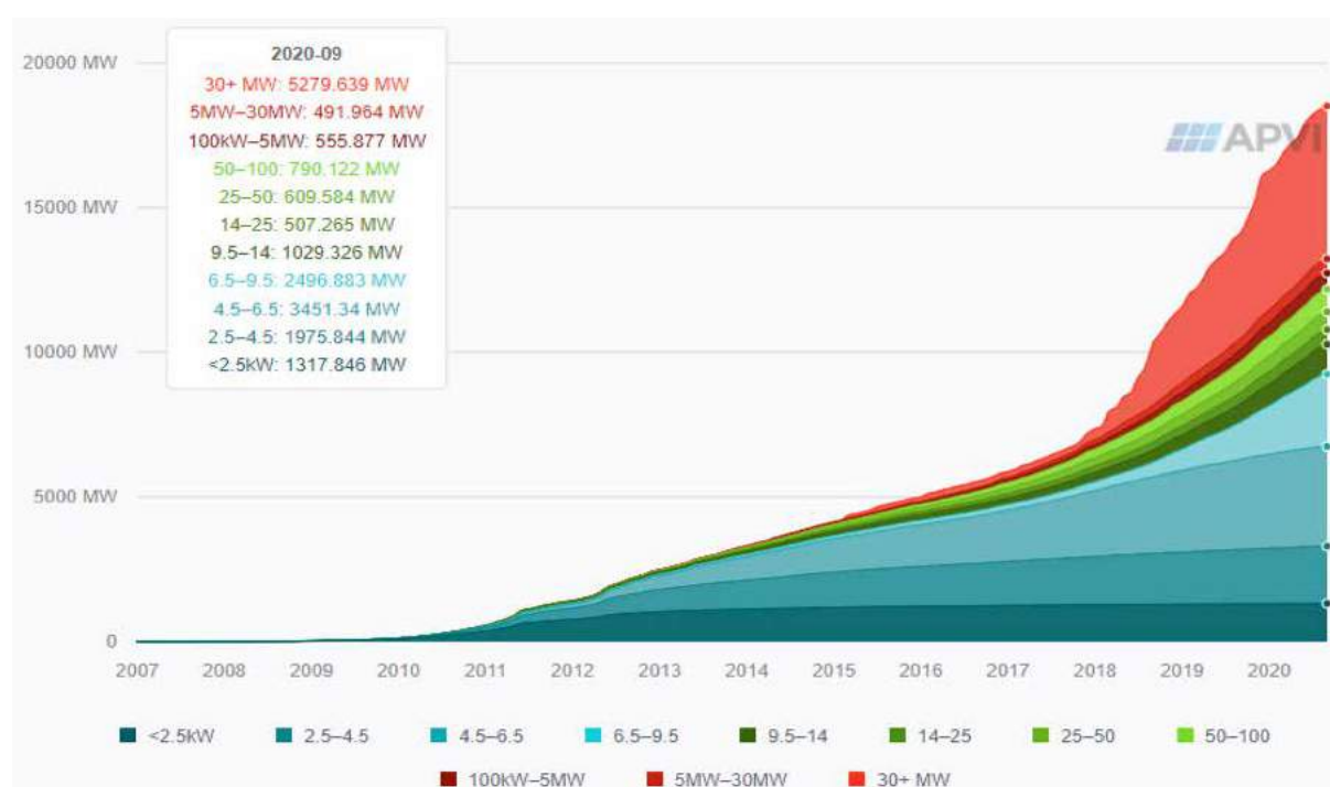
Fig. 2 - Cumulative installed capacity by system size to end of September 2020.
