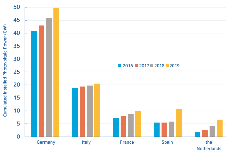
Fig. 1 - Cumulative installed photovoltaic capacity in some EU countries [8].
