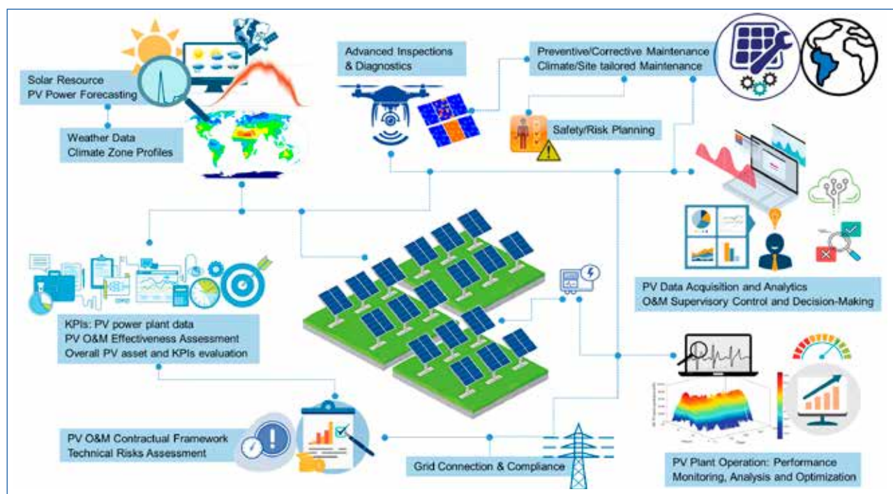
Fig. 4 – Overview of operation & maintenance aspects and services for PV power systems during their technical lifecycle (source: CEA-INES). This ST3.3 Report “Guidelines for Operation and Maintenance in Different Climates” will be published in 2021.
