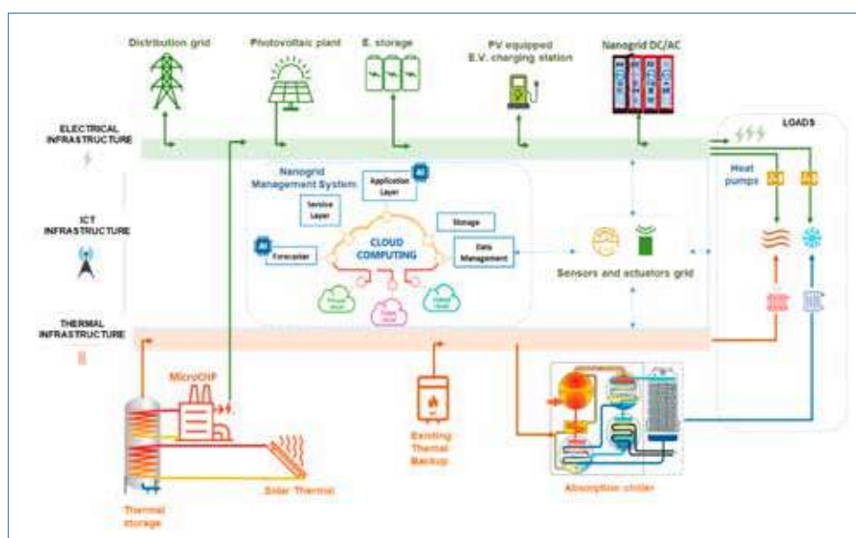
Fig. 3 - ENEA experimental multivector smart nanogrid layout.
