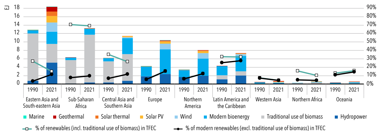
FIGURE 3.6 • RENEWABLE ENERGY CONSUMPTION AND SHARE IN TFEC BY REGION, 1990 AND 2021
