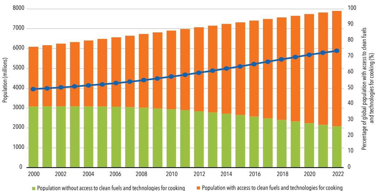
FIGURE 2.4 • CHANGE IN THE ABSOLUTE NUMBER OF PEOPLE (LEFT AXIS, BARS) AND PERCENTAGE OF THE GLOBAL POPULATION (RIGHT AXIS, LINE) WITH ACCESS TO CLEAN COOKING, 2000–22
