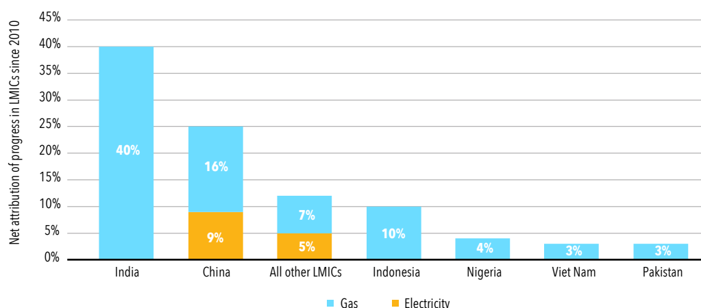
FIGURE 2.13 • BREAKDOWN OF PROGRESS TOWARD UNIVERSAL ACCESS TO CLEAN COOKING IN LMICS SINCE 2010 BY FUEL
