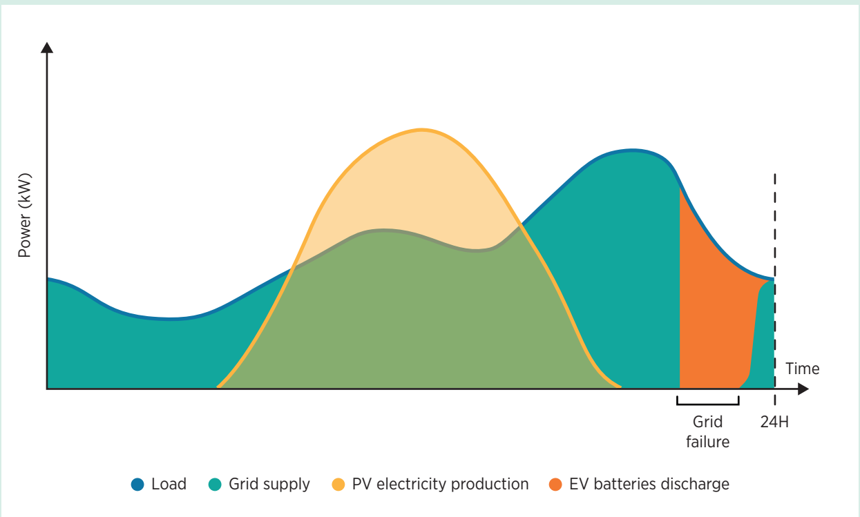
Figure 16: Effect of EV battery used as a back-up for the grid
