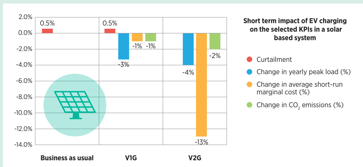
Figure S5: Short-term impact of EV charging
