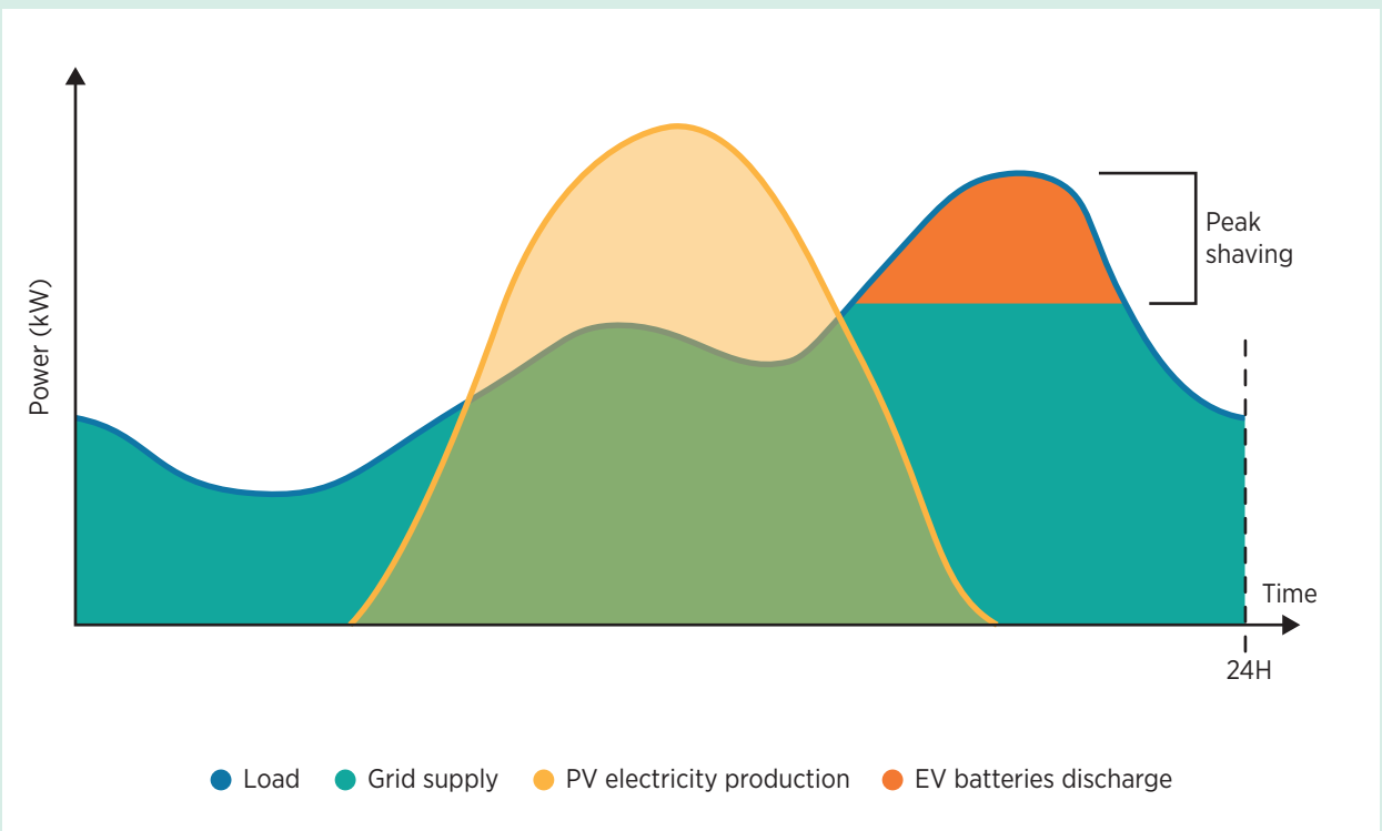
Figure 17: Effect of peak shaving
