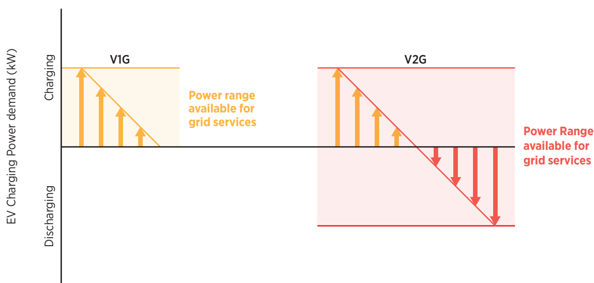
Figure 14: Example of unidirectional (V1G) versus bidirectional (V2G) grid services provision
