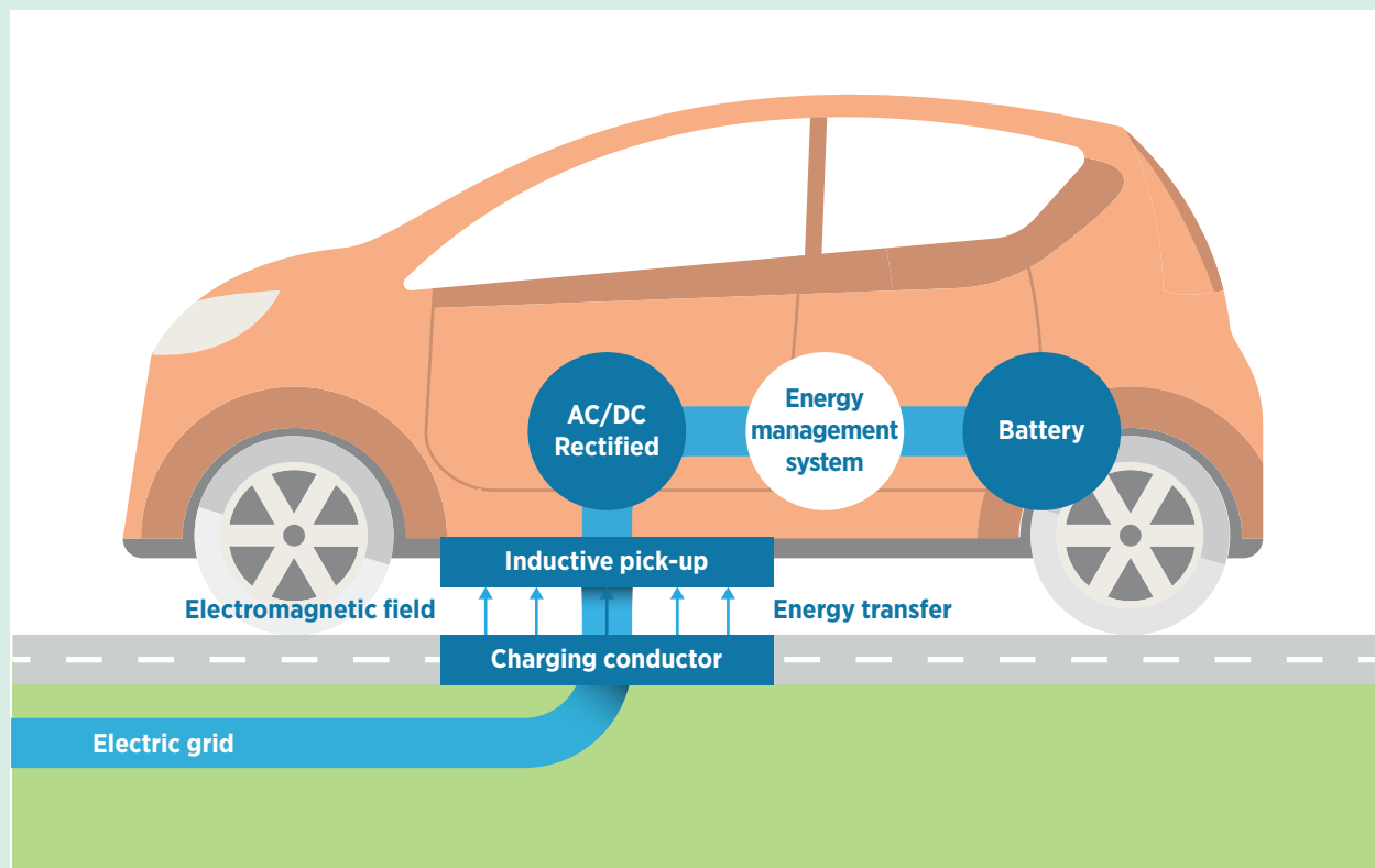
Figure 19: Inductive charging
