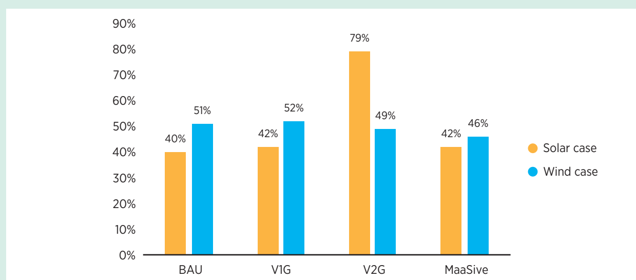
Figure 34: Renewable shares in generation in wind- and solar-based systems under different charging scenarios (long-term impact)*
