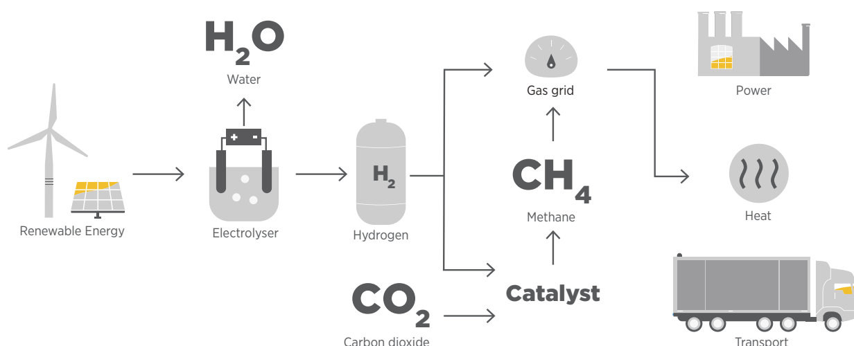
FIGURE 51: Power-to-gas process
