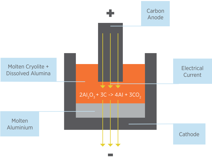
FIGURE 30: Schematic representation of the Hall-Hérout process
