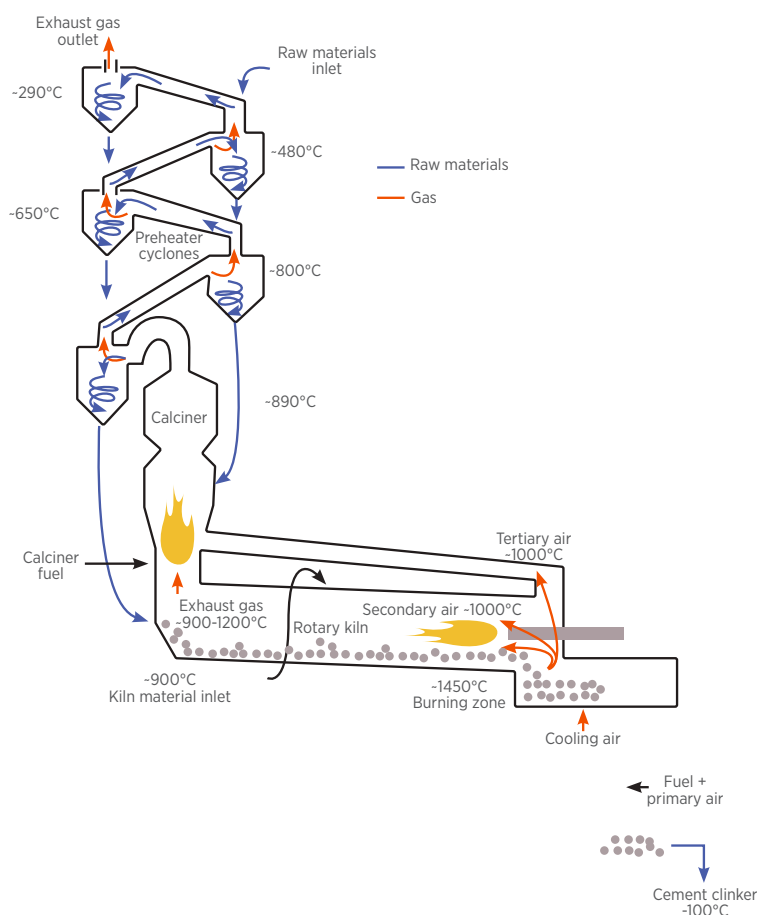
FIGURE 26: Schematic of an example cement kiln
