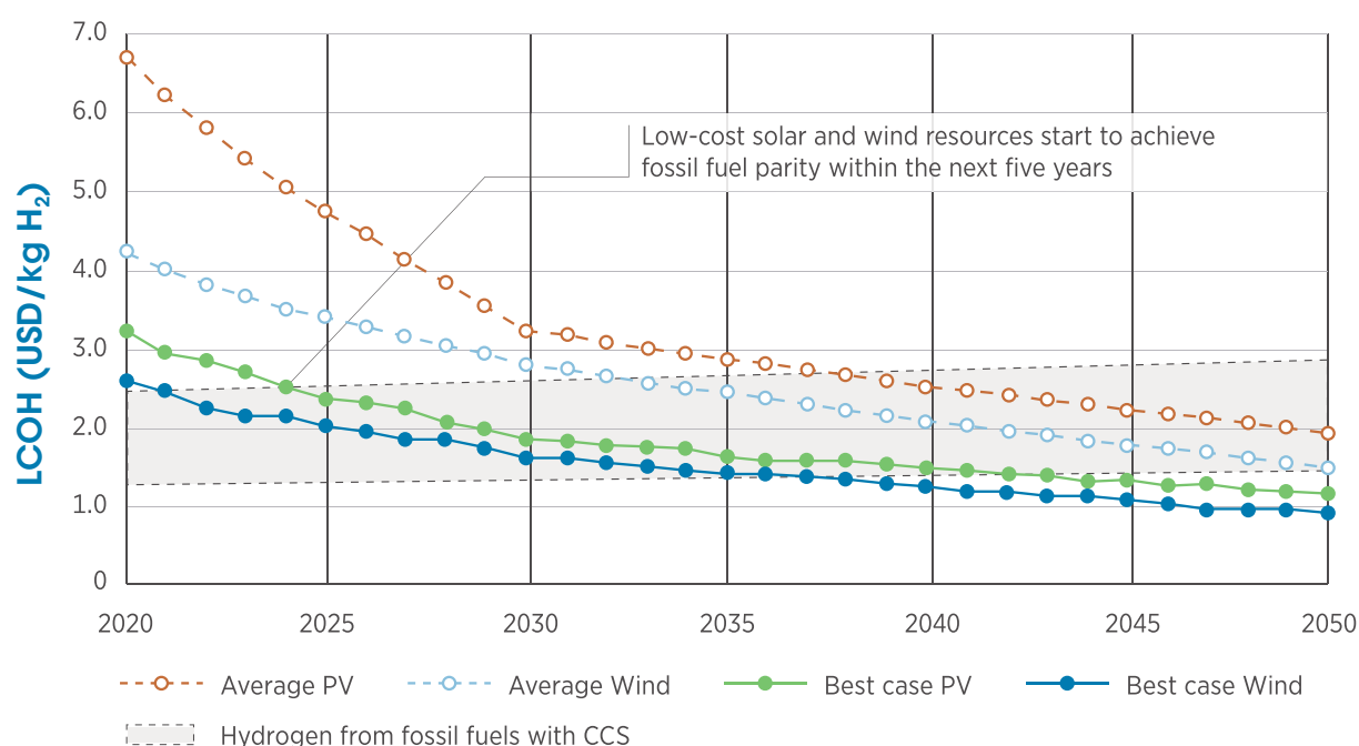
FIGURE 49: Green hydrogen production cost projections
