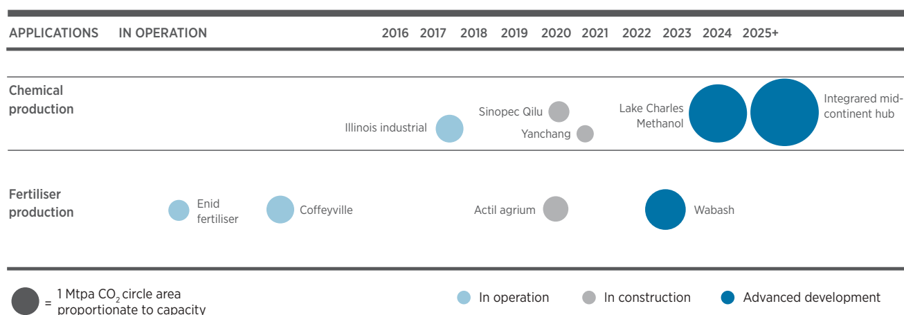
FIGURE 20: Large-scale CCUS facilities in operation, construction and development for chemical or fertiliser production
