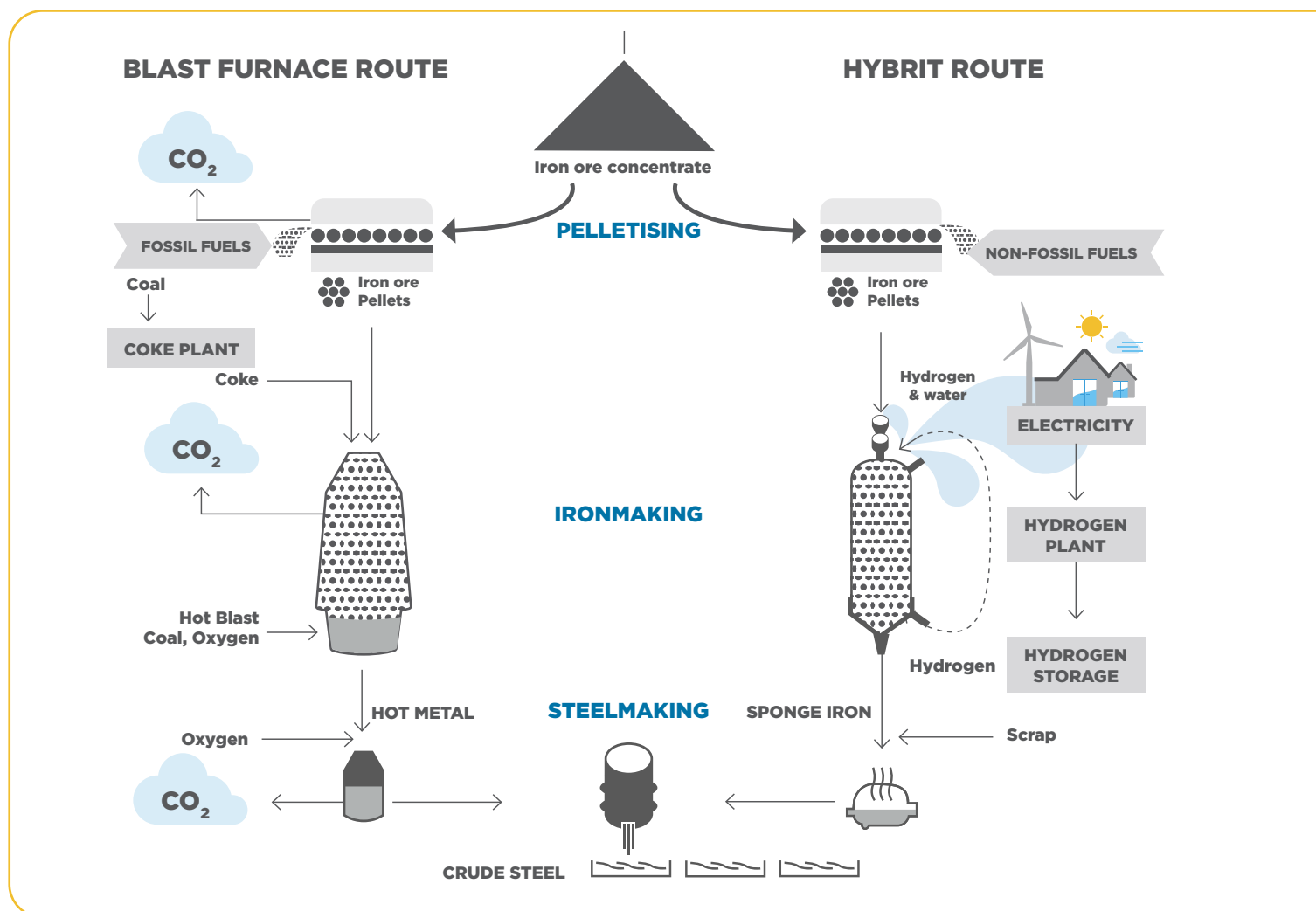
FIGURE 11: Renewable hydrogen-based DRI-EAF route piloted in Sweden compared to the conventional BF-BOF route
