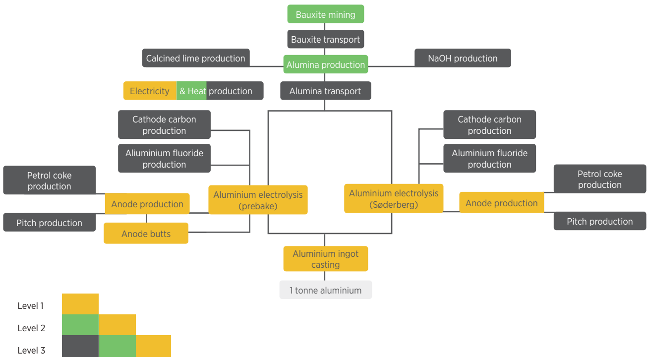
FIGURE 31: Processes in the primary aluminium production chain
