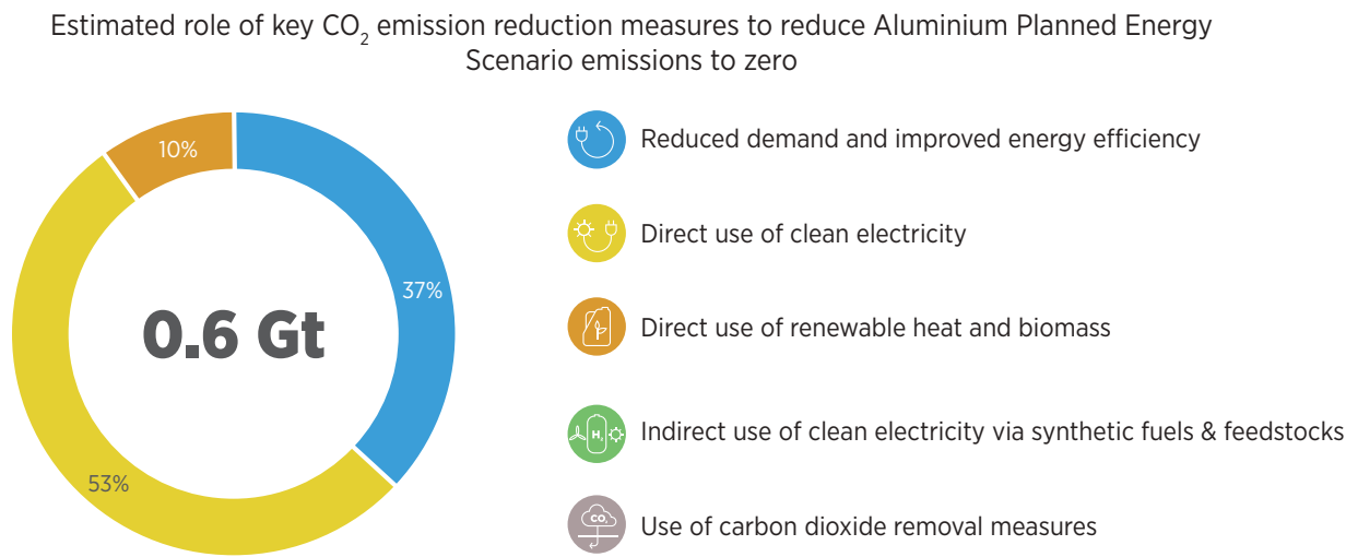
FIGURE 28: Emission reduction measures to reach zero emissions in the aluminium sector, from Planned Energy Scenario to zero
