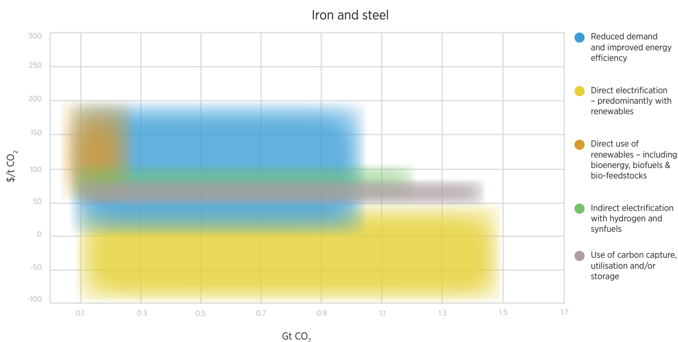
FIGURE 8: Estimated abatement potential of measures to reach zero energy emissions in the iron and steel sector plotted against estimates of the cost of abatement
