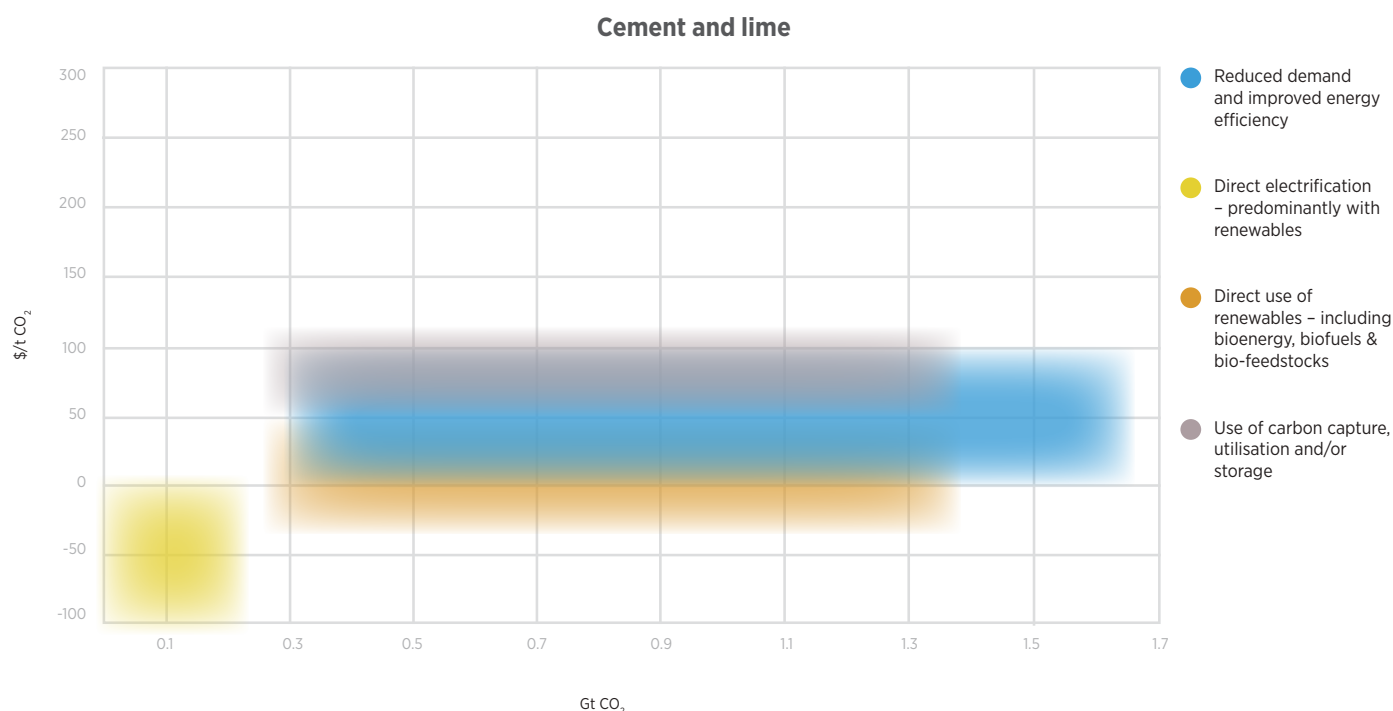
FIGURE 23: Estimated abatement potential of measures to reach zero energy emissions in the cement and lime sector plotted against estimates of the cost of abatement
