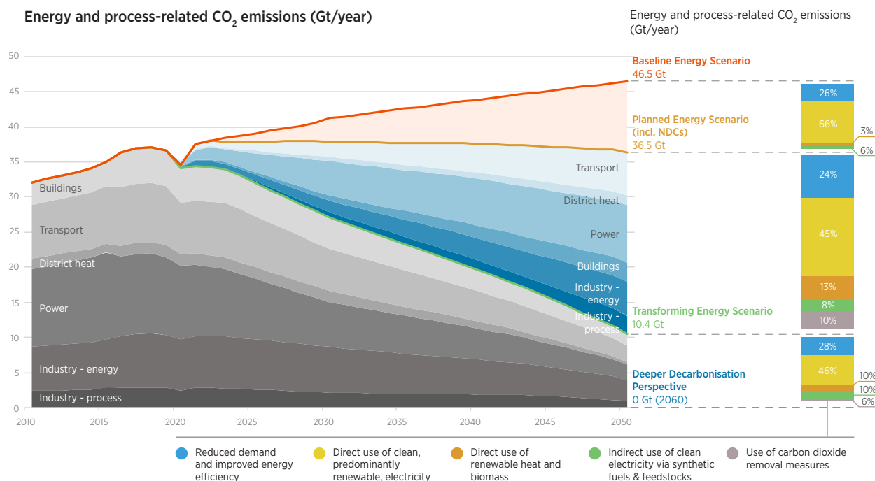
FIGURE 1: Energy- and process-related CO 2 annual emissions trajectories from 2010 till 2050
