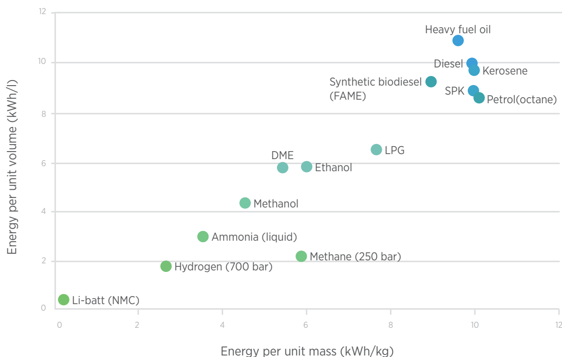
FIGURE 42: Volumetric and gravimetric densities of potential transport fuels
