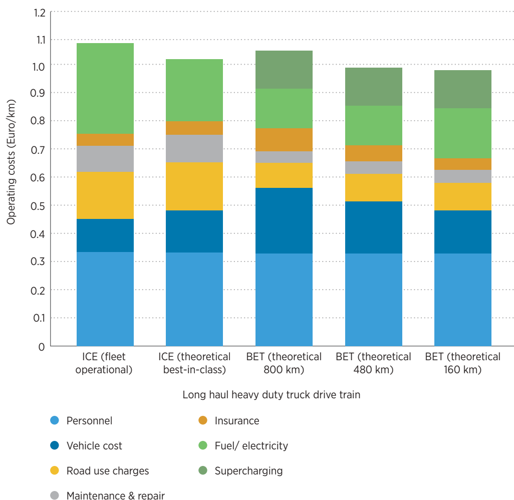
FIGURE 37: Five-year total cost of ownership comparison for diesel and battery electric trucks
