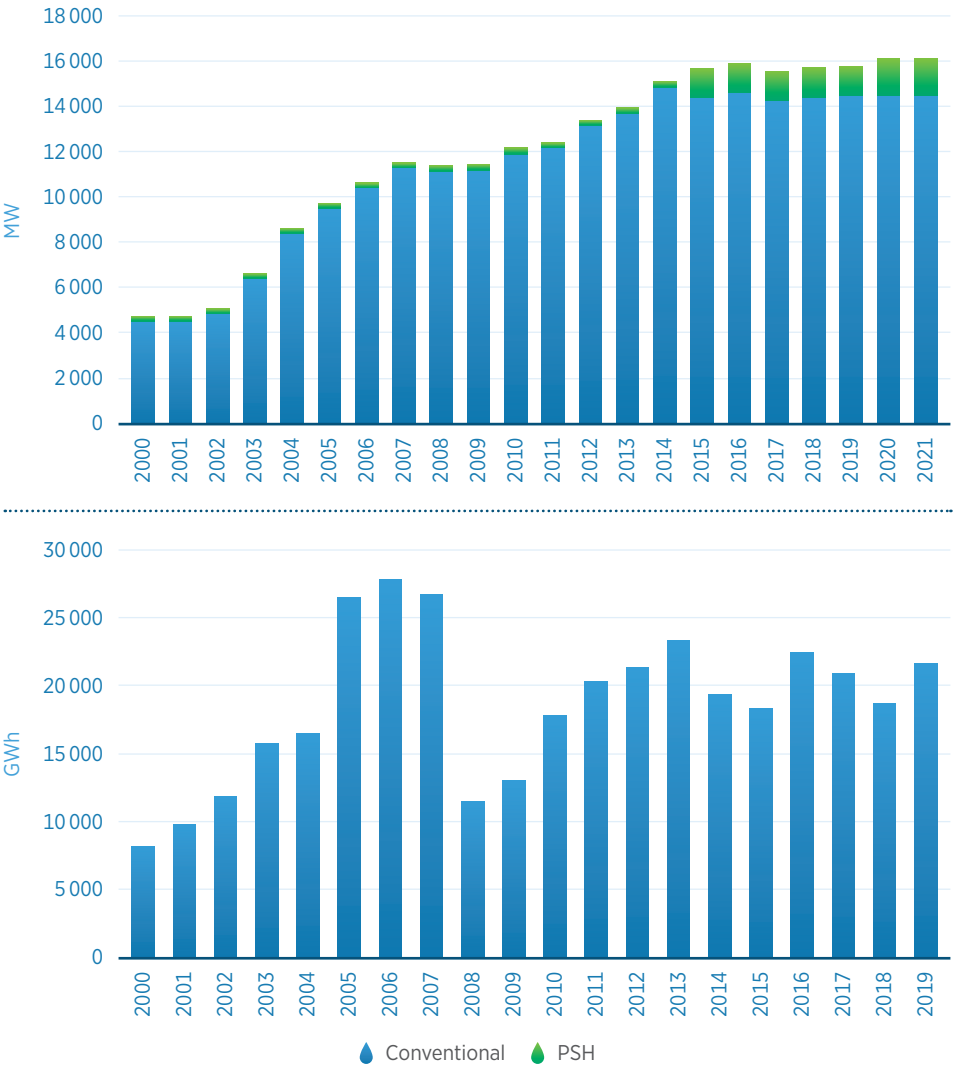
Figure B.21 Hydropower capacity and generation in the Middle East, 2000-2021
