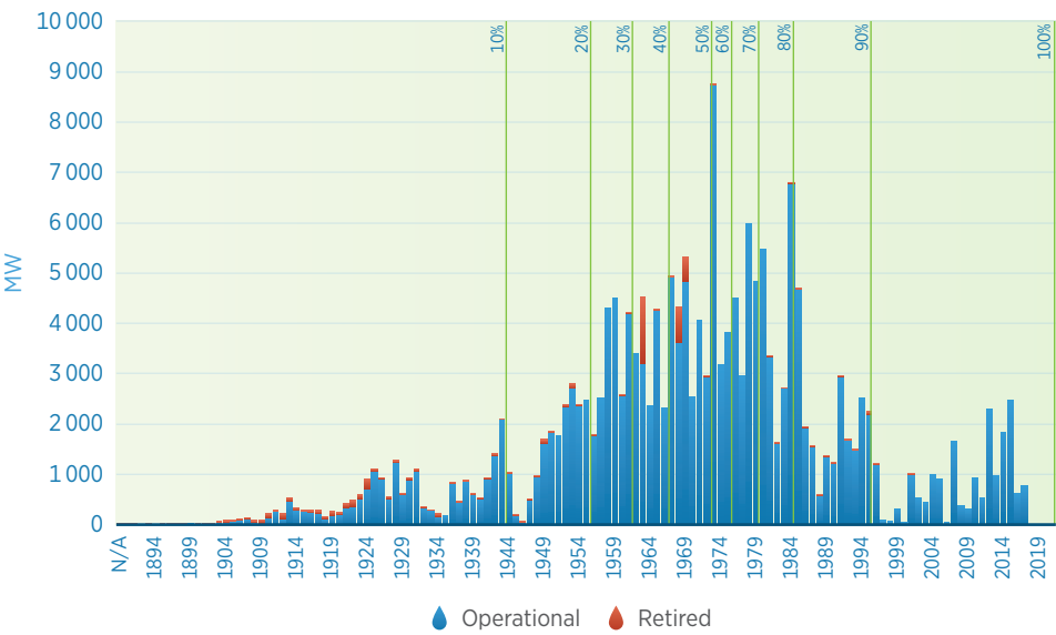
Figure B.28 Hydropower capacity in North America by year of commissioning
