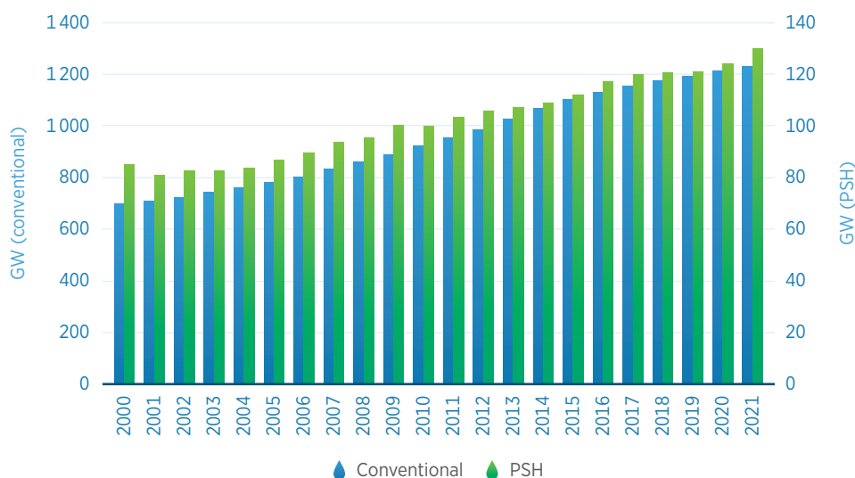
Figure 3 Hydropower installed capacity by year, 2000-2021
