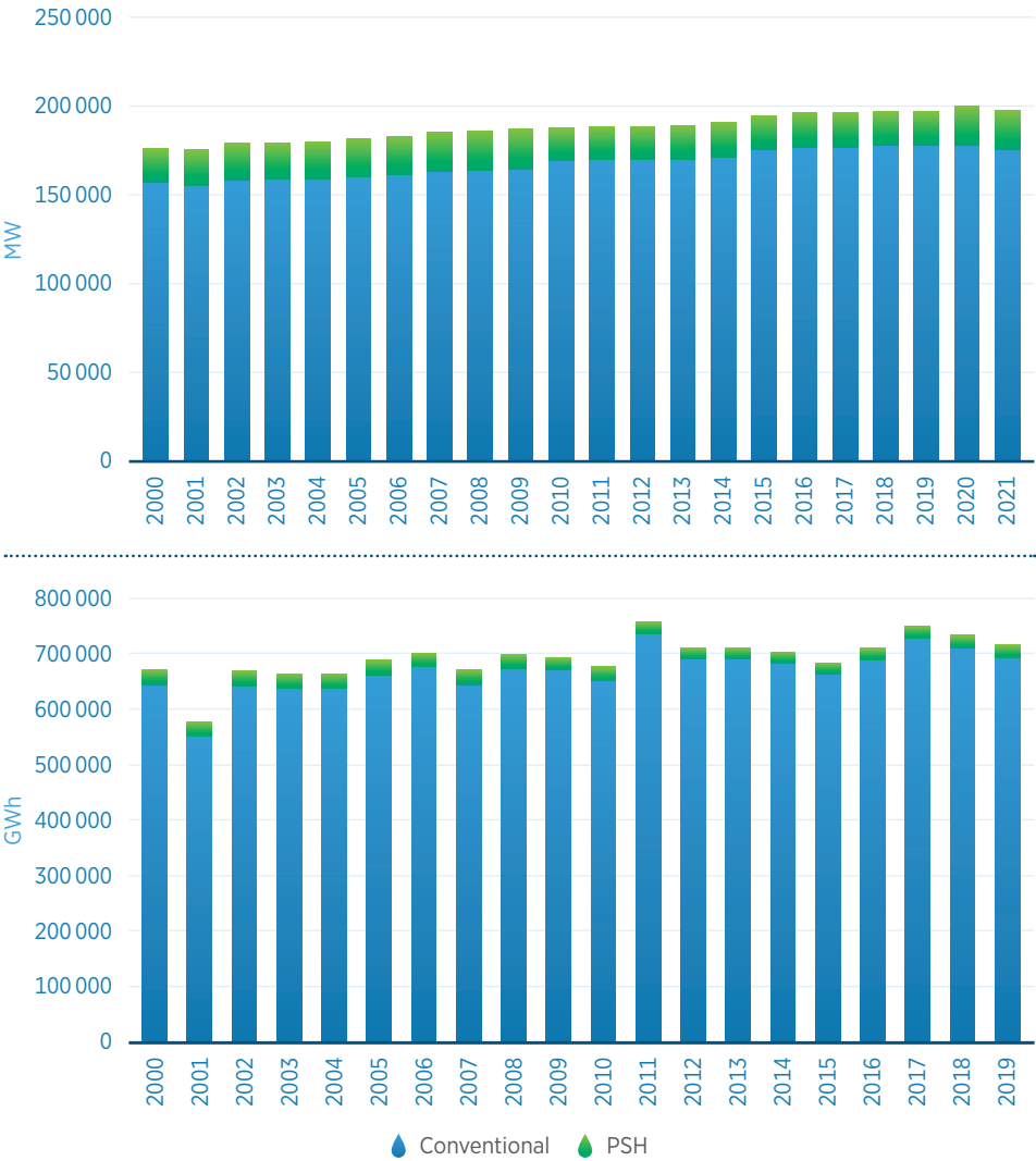
Figure B.25 Hydropower capacity and generation in North America, 2000-2021
