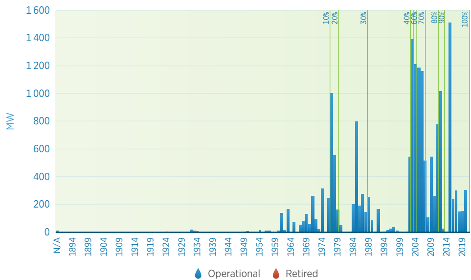
Figure B.24 Hydropower capacity in the Middle East by year of commissioning
