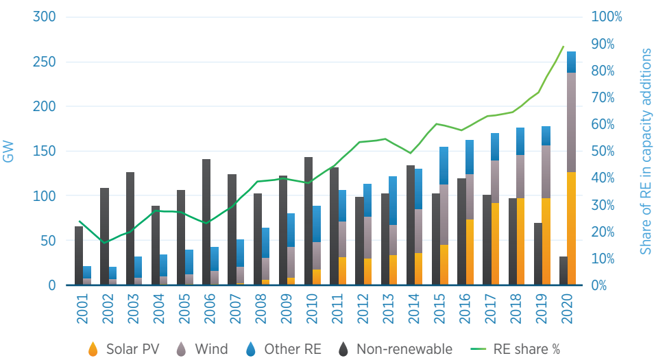
Figure 14 Comparison of renewable and non-renewable net capacity additions, 2001-2020
