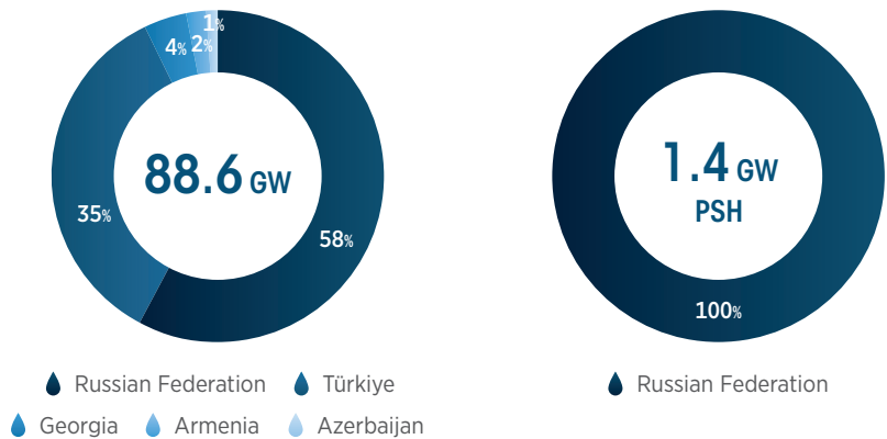
Figure B.14 Hydropower installed capacity in Eurasia, 2021
