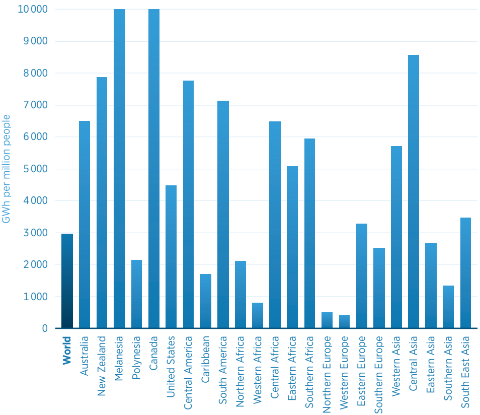
Figure 2 Energy storage potential by region
