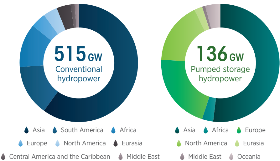
Figure 6 Hydropower project pipeline, 2022-2037
