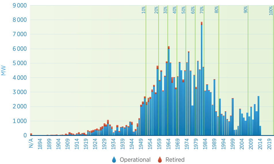
Figure B.20 Hydropower capacity in Europe by year of commissioning
