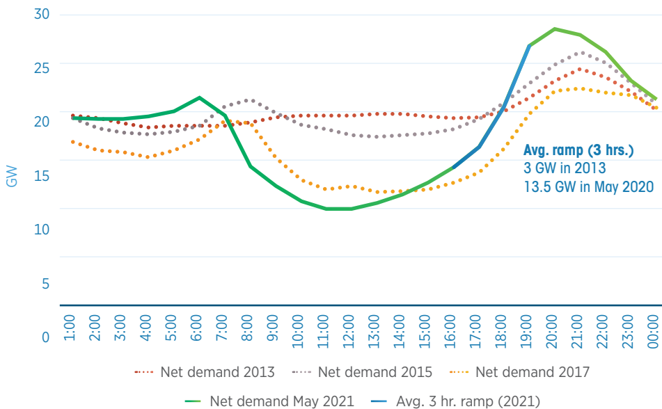
Figure 15 Net demand curve for a spring day in California in 2020
