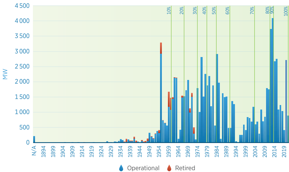
Figure B.16 Hydropower capacity in Eurasia by year of commissioning
