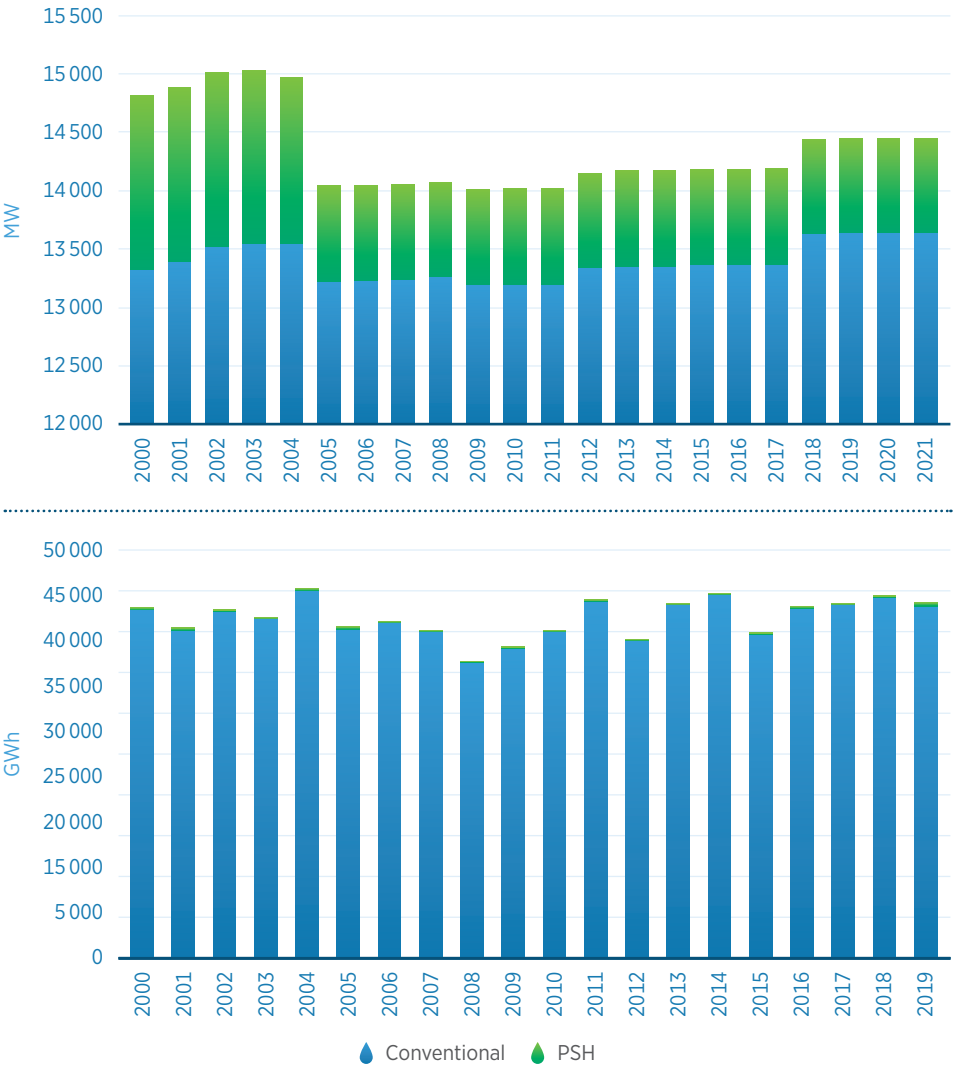
Figure B.29 Hydropower capacity and generation in Oceania, 2000-2021
