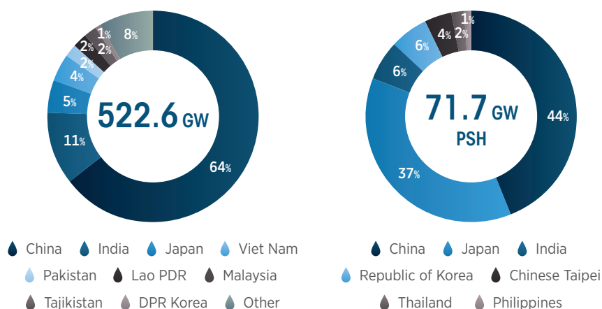
Figure B.6 Hydropower installed capacity in Asia, 2021
