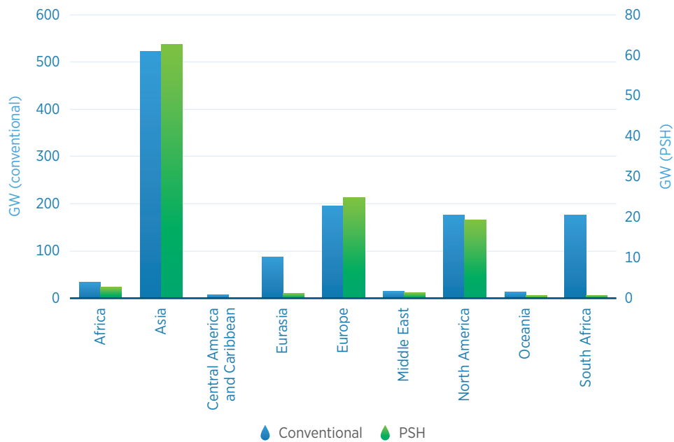
Figure 4 Hydropower installed capacity by region, 2021
