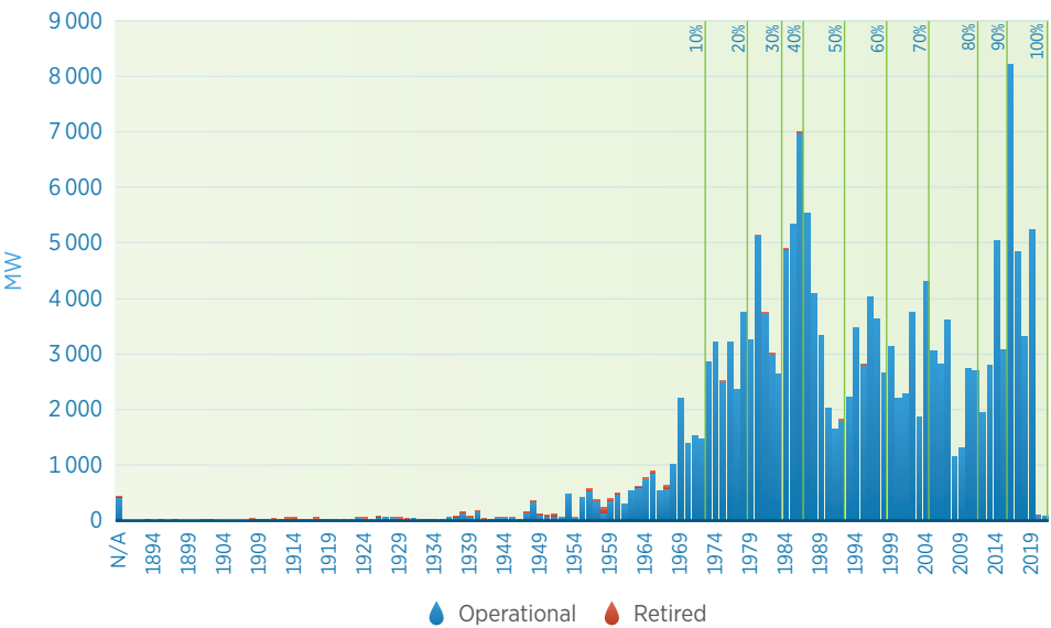
Figure B.36 Hydropower capacity in South America by year of commissioning
