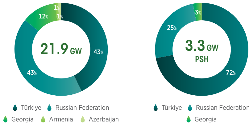
Figure B.15 Hydropower project pipeline in Eurasia, 2022-2037
