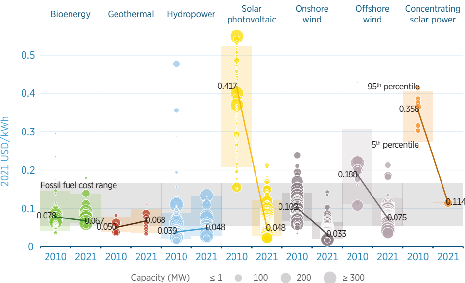
Figure 8 Levelised cost of electricity for utility-scale renewable power generation, global weighted average, 2010-2021
