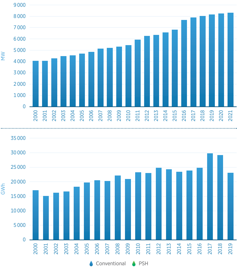
Figure B.9 Hydropower capacity and generation in Central America and the Caribbean, 2000-2021
