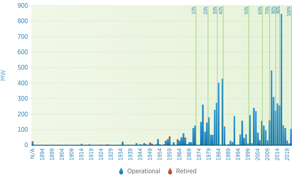
Figure B.12 Hydropower capacity in Central America and the Caribbean by year of commissioning
