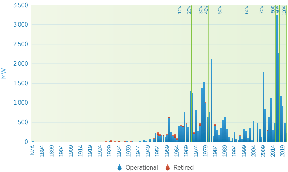
Figure B.4 Hydropower capacity in Africa by year of commissioning
