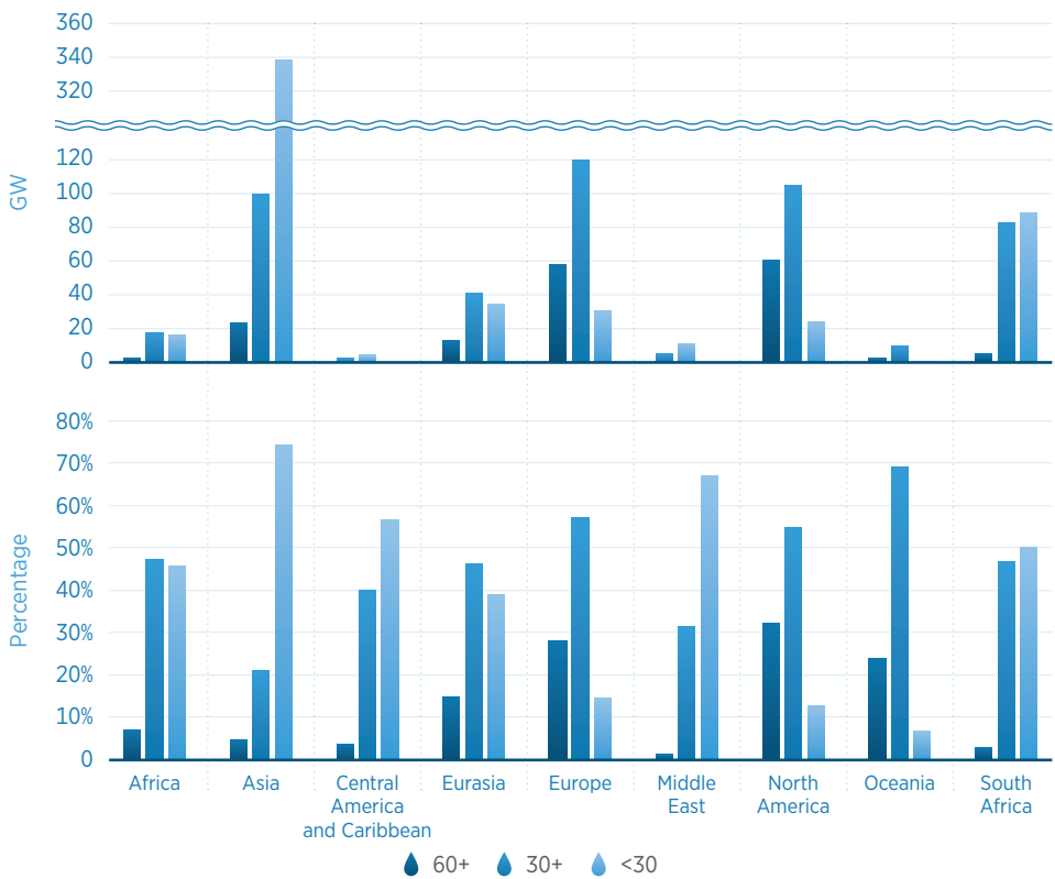
Figure 12 Breakdown of hydropower fleet age by region
