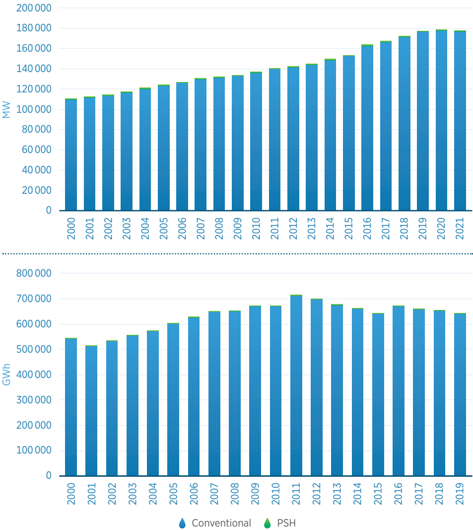
Figure B.33 Hydropower capacity and generation in South America, 2000-2021
