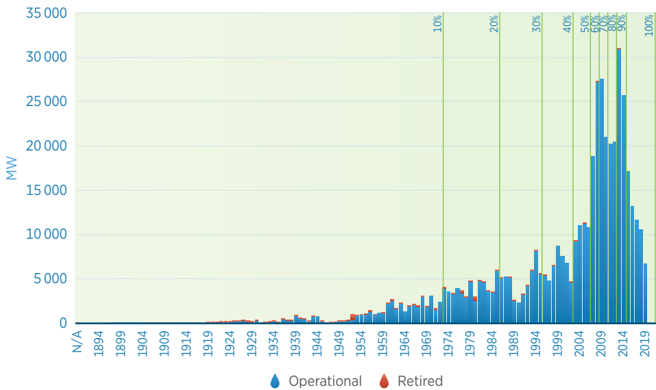
Figure B.8 Hydropower capacity in Asia by year of commissioning
