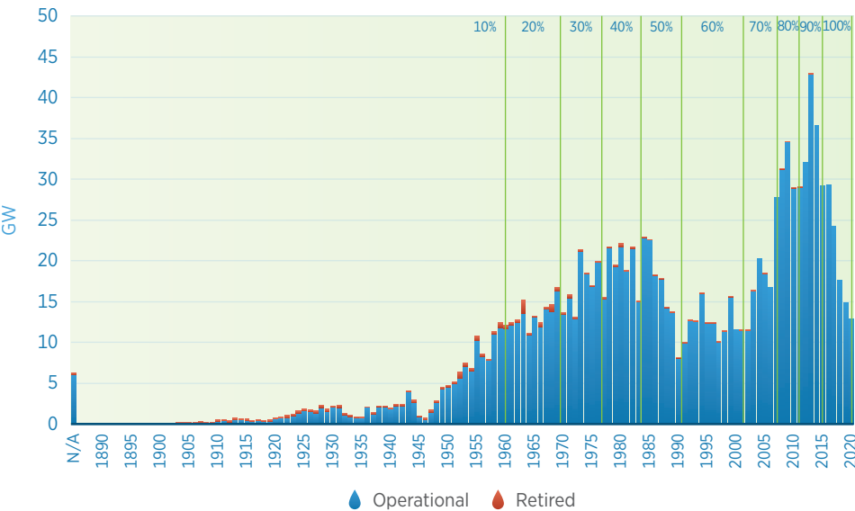
Figure 11 Global hydropower capacity by year of commissioning
