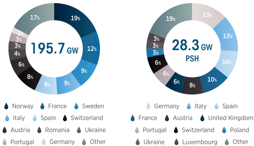
Figure B.18 Hydropower installed capacity in Europe, 2021
