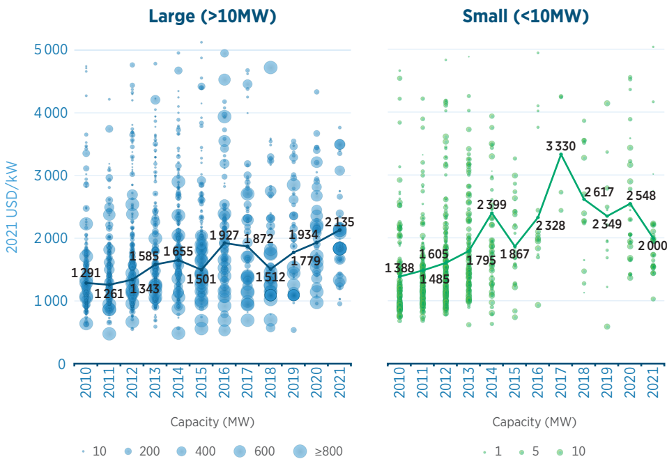
Figure 7 Hydropower’s total installed costs, global weighted average, 2010-2021
