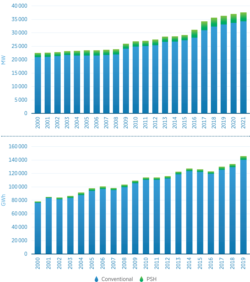
Figure B.1 Hydropower capacity and generation in Africa, 2000-2021
