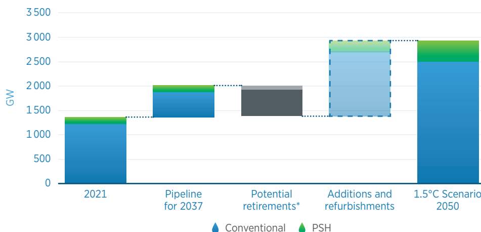
Figure 13 Necessary hydropower capacity additions by 2050
