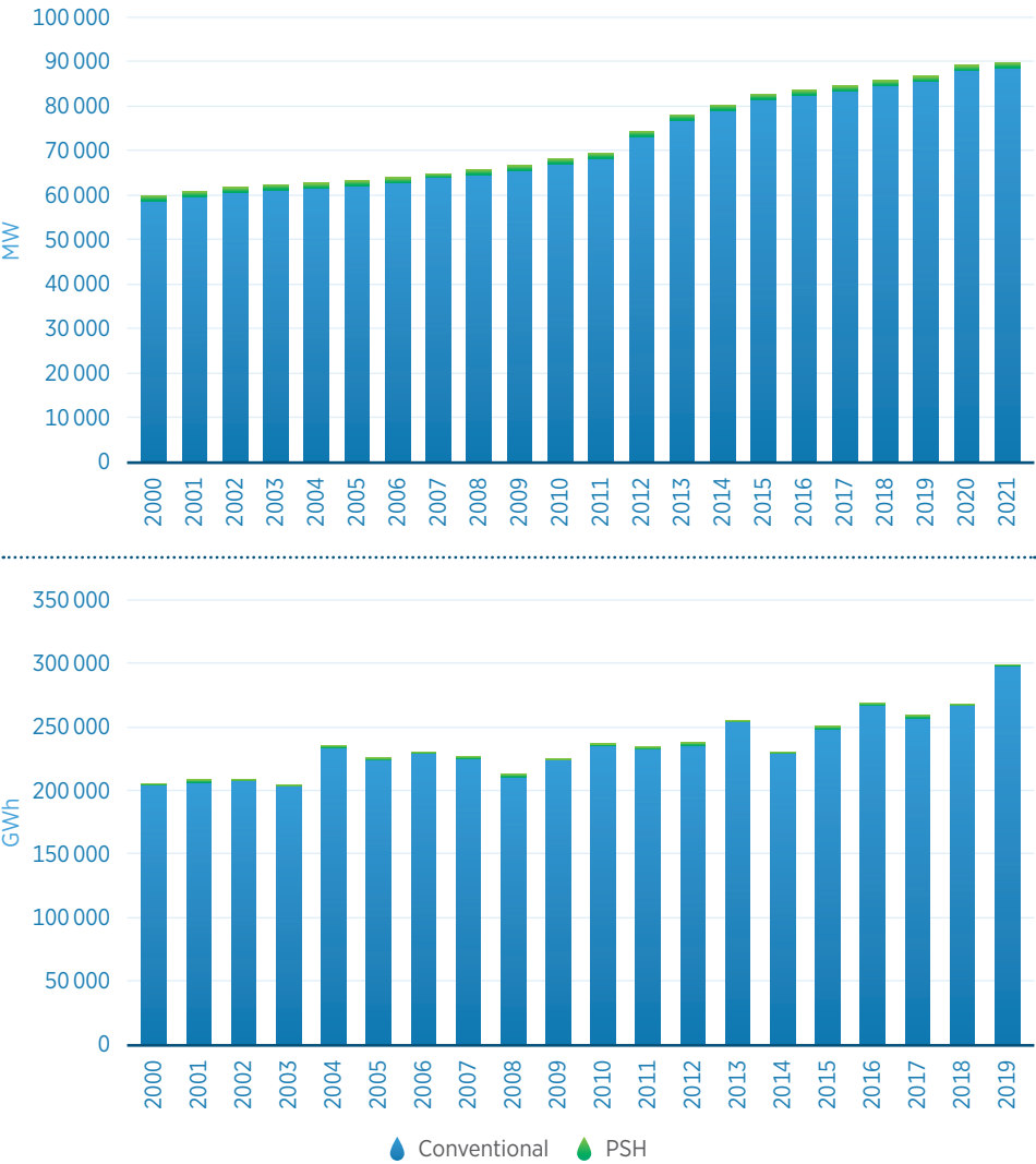
Figure B.13 Hydropower capacity and generation in Eurasia, 2000-2021
