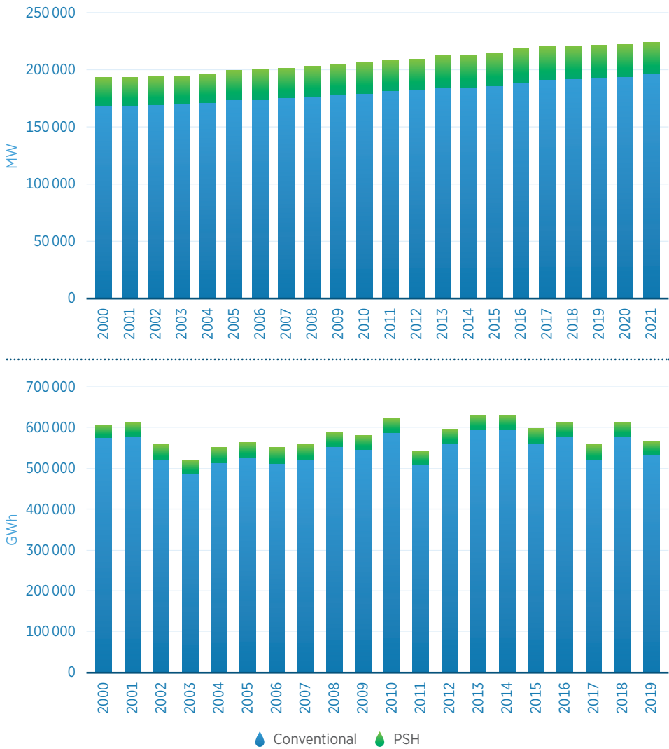
Figure B.17 Hydropower capacity and generation in Europe, 2000-2021
