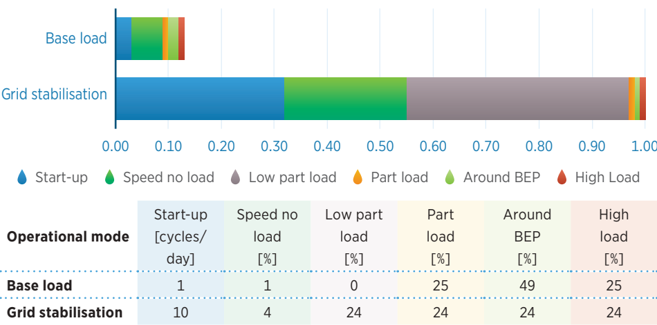
Figure 16 Relative operational damage contributions to a Francis turbine
