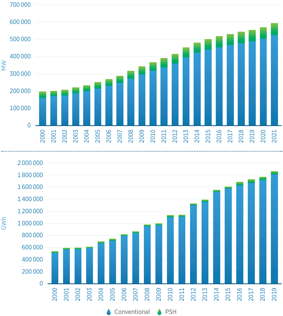
Figure B.5 Hydropower capacity and generation in Asia, 2000-2021
