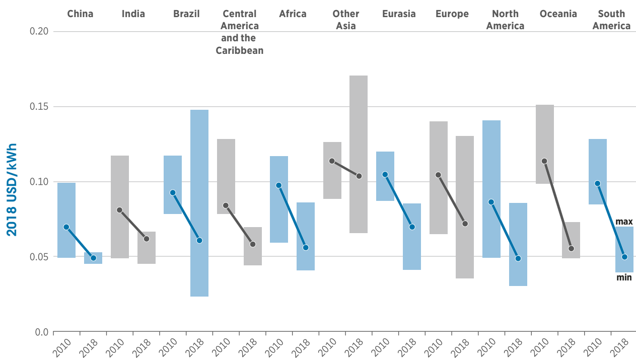
Figure 13: Regional weighted average levelised cost of electricity and ranges for onshore wind in 2010 and 2018.
