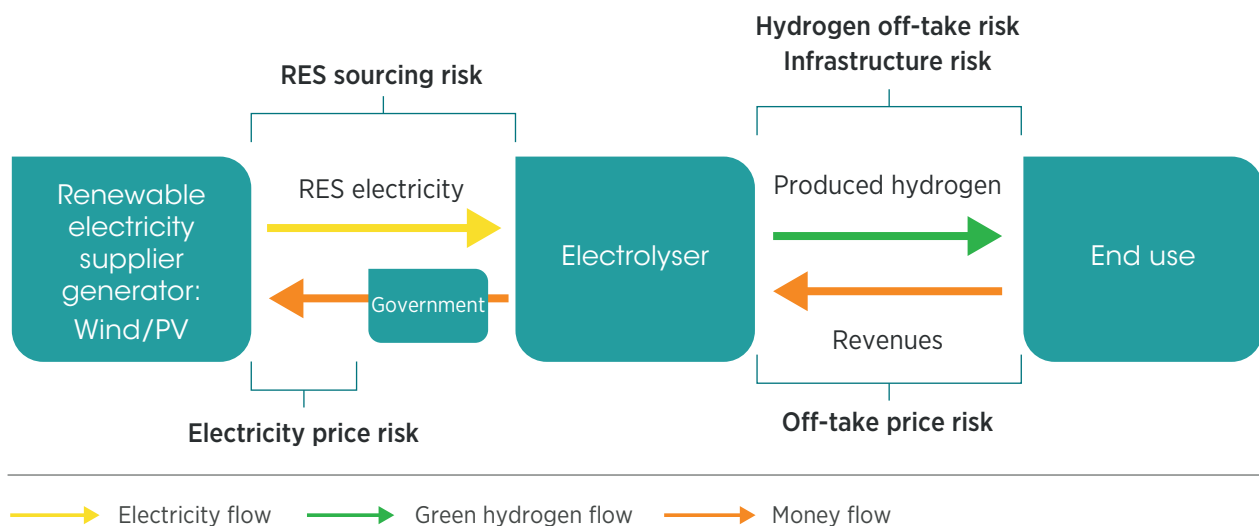
Figure 9 Hydrogen value chain with government assuming electricity price risk
