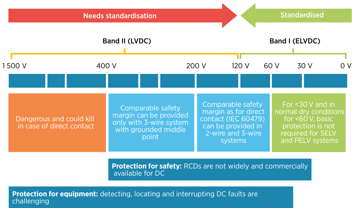
Figure 53 DC mini-grid standardisation needs by nominal voltage level 3
