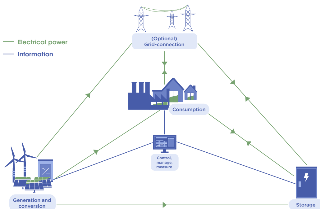
Figure 13 Mini-grid functionalities
