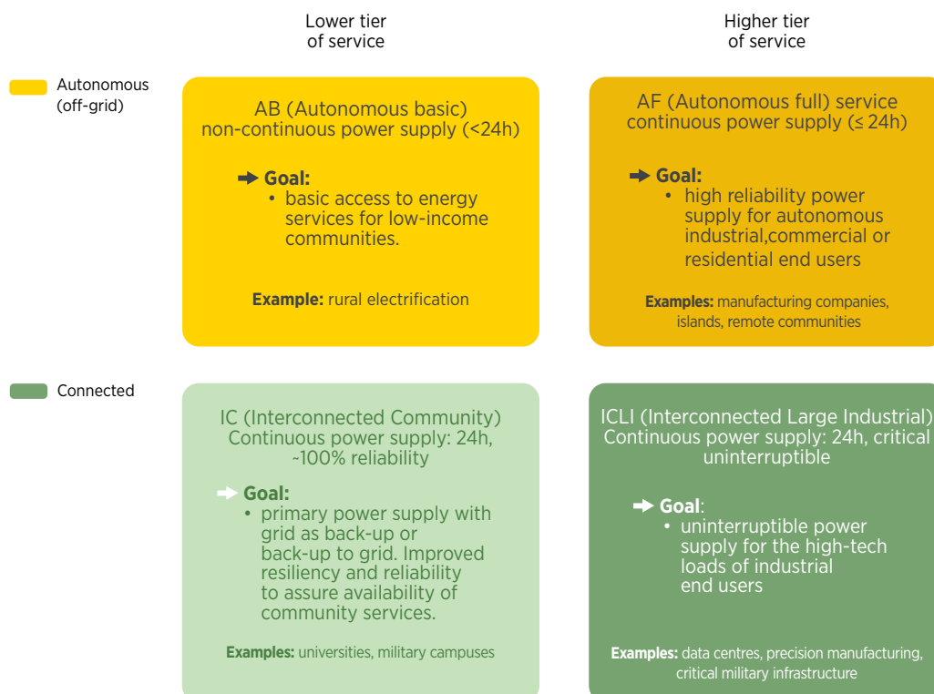
Figure 14 Mini-grid types
