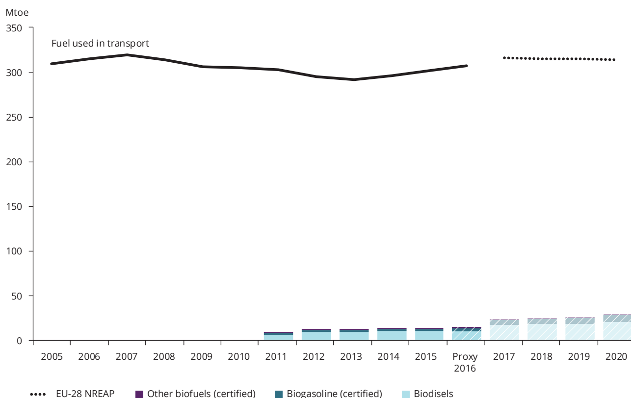
Figure 2.14 Renewable transport in the EU-28: biofuels
