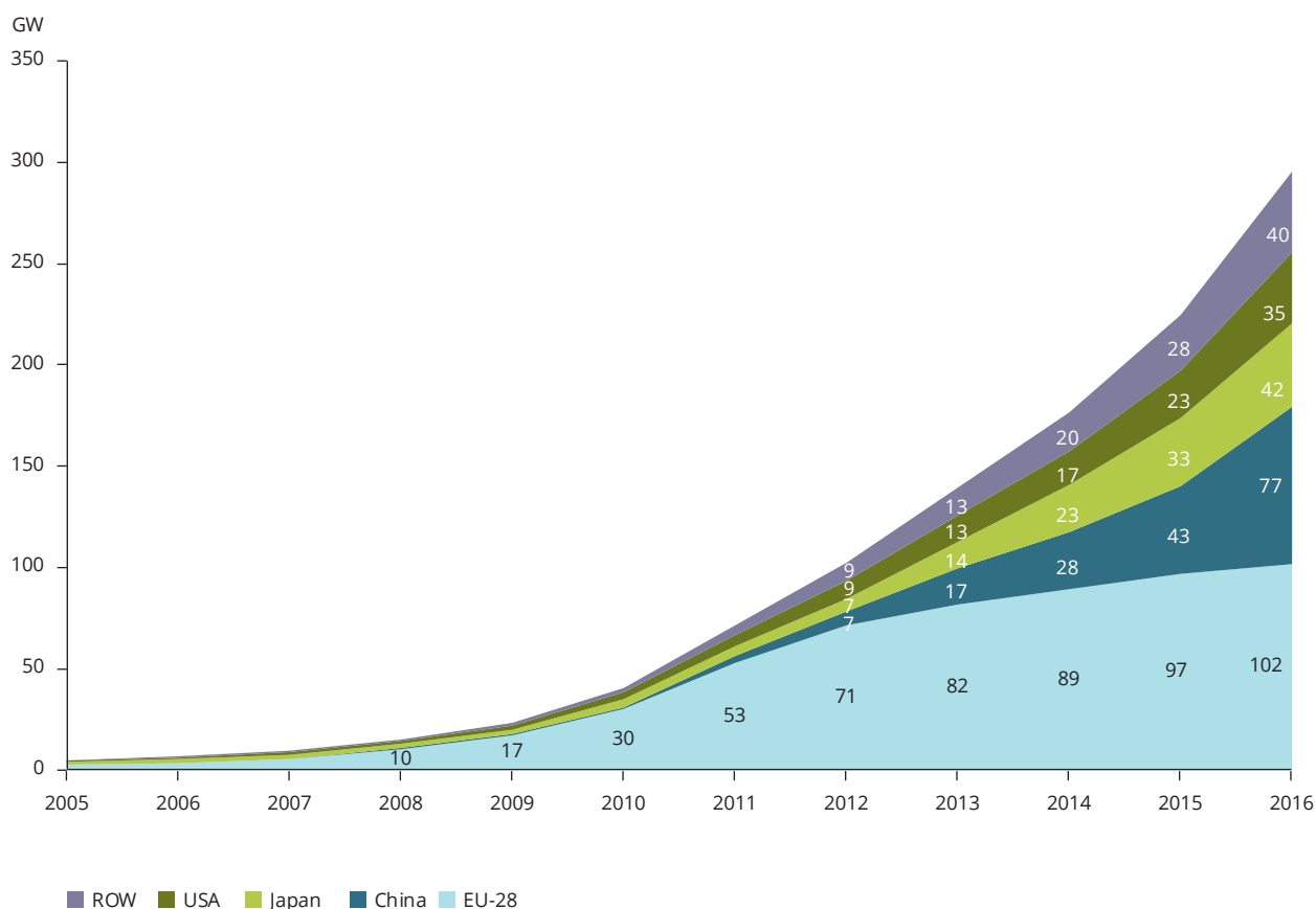
Figure 4.4 Growth in total solar PV capacity in the EU-28, the top three countries and the rest of the world (ROW), 2005-2016
