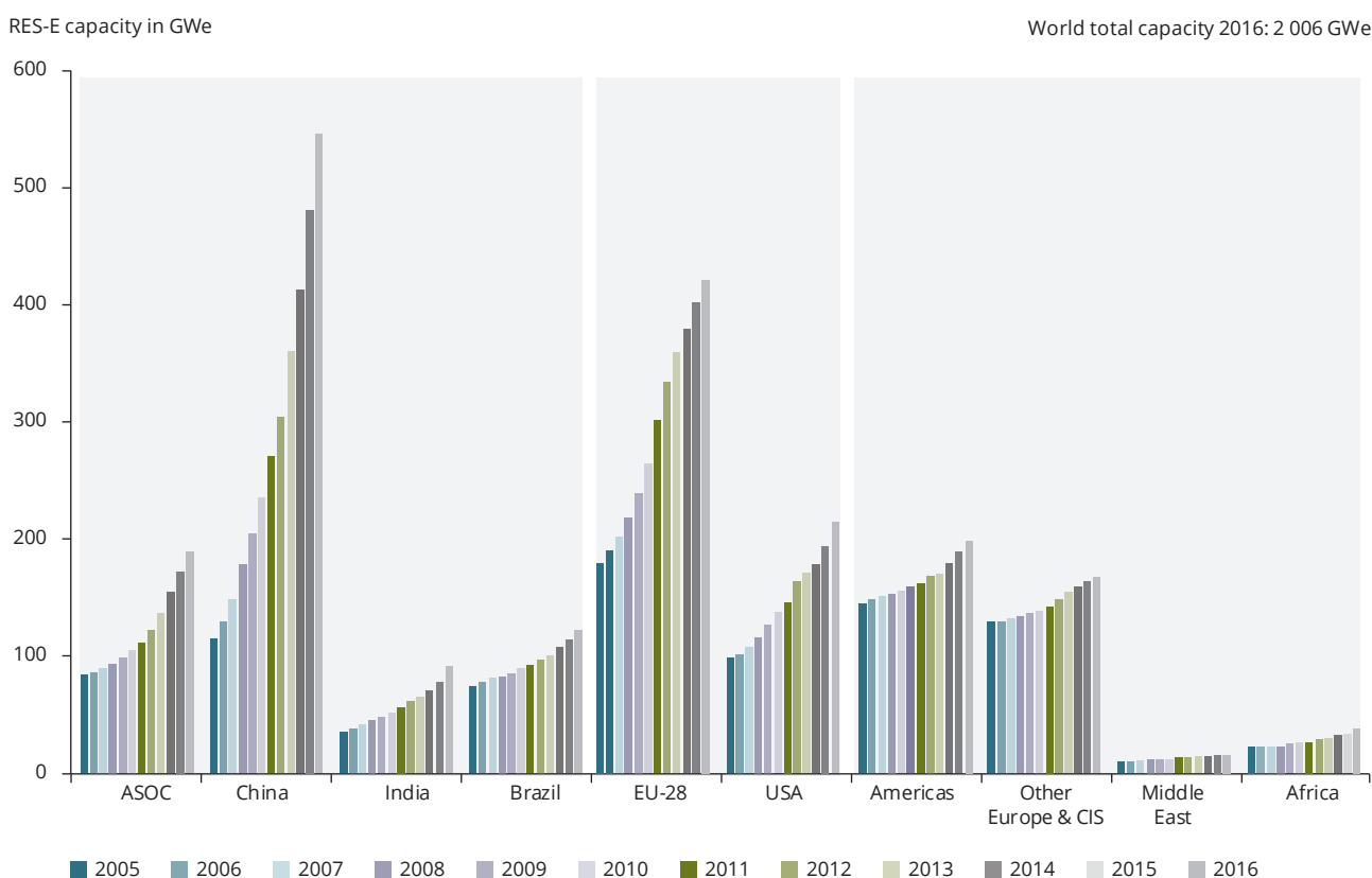
Figure 4.1 RES-E capacities in selected world regions, 2005-2016
