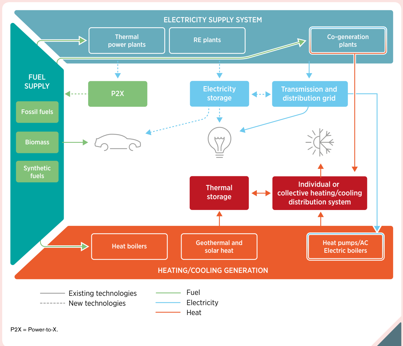
Figure 5.5. Sector coupling
