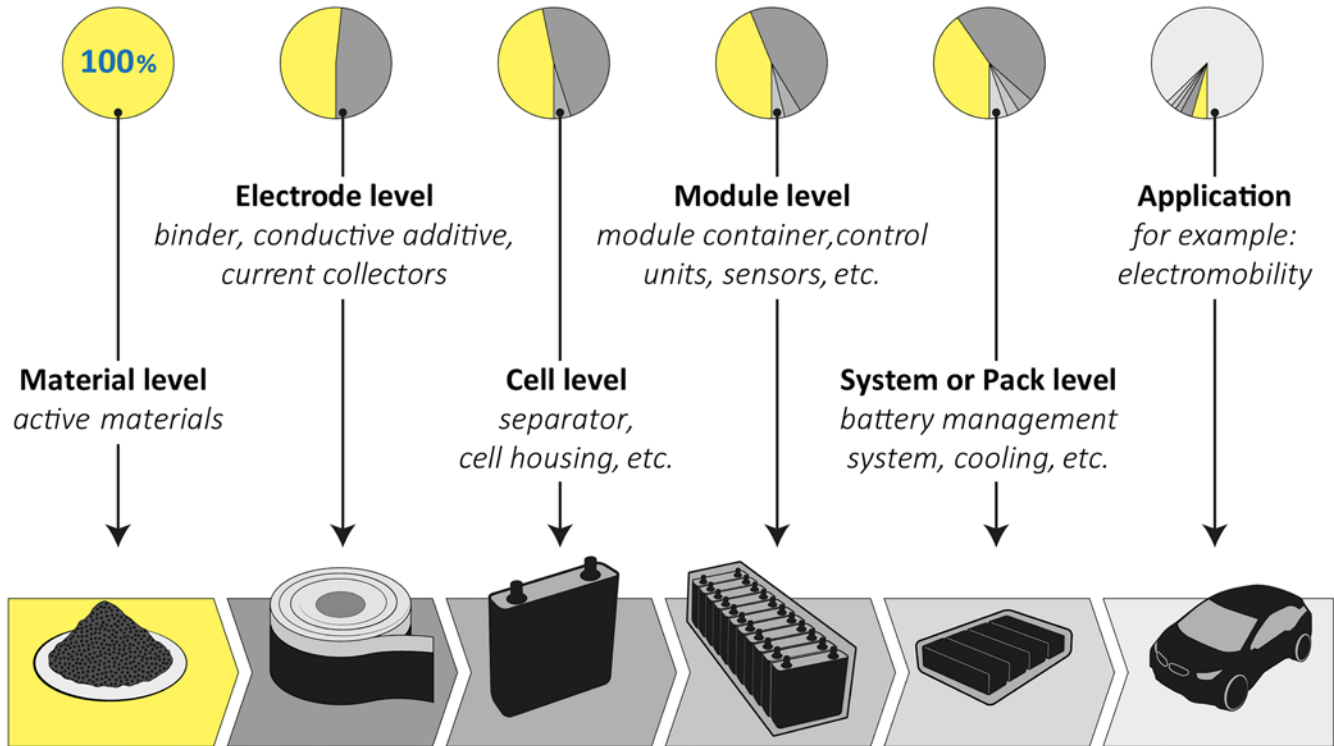
Figure 2. Schematic illustration of a battery's production chain, from the material level via the battery cell, to the battery system level. In each step, inactive components are added and assembled into a key 'building block' for the battery system, which 'dilute' the energy provided by the active materials.
