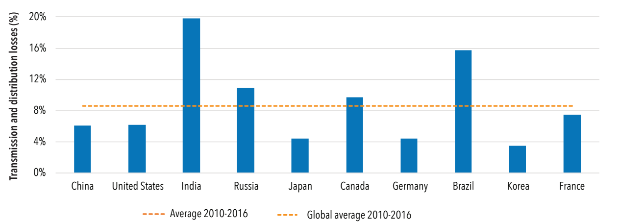
FIGURE 4.9 • TRANSMISSION AND DISTRIBUTION LOSSES FOR THE WORLD’S 10 LARGEST ELECTRICITY PRODUCERS, 2016
