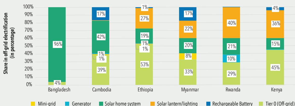
FIGURE B1.2.1 • OFF-GRID SOLUTIONS IN BANGLADESH, CAMBODIA, ETHIOPIA, MYANMAR, KENYA AND RWANDA, BY TECHNOLOGY, 2017
