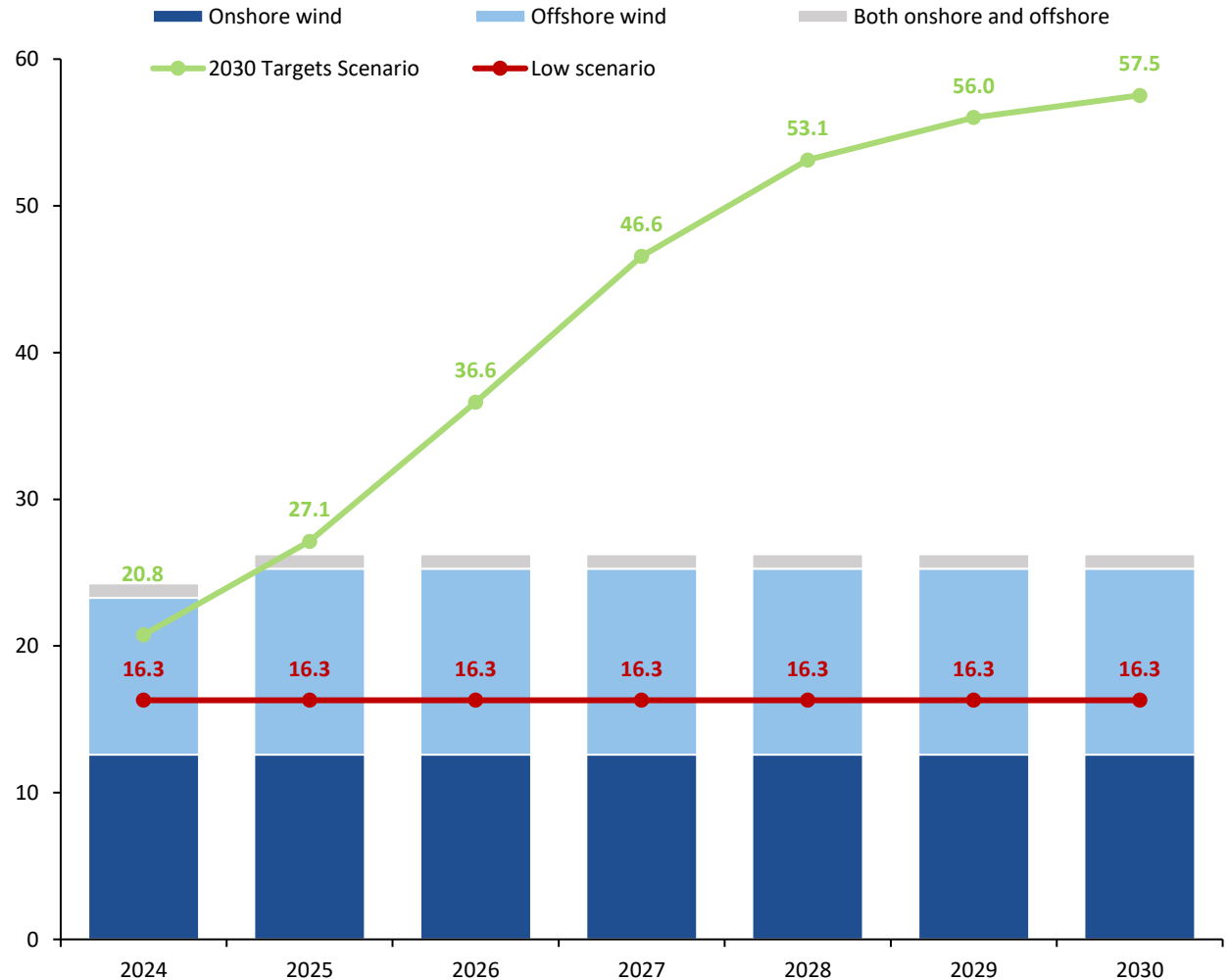
Figure 39: Turbine manufacturing capacity, annual capacity additions, Europe Gigawatts (GW)
